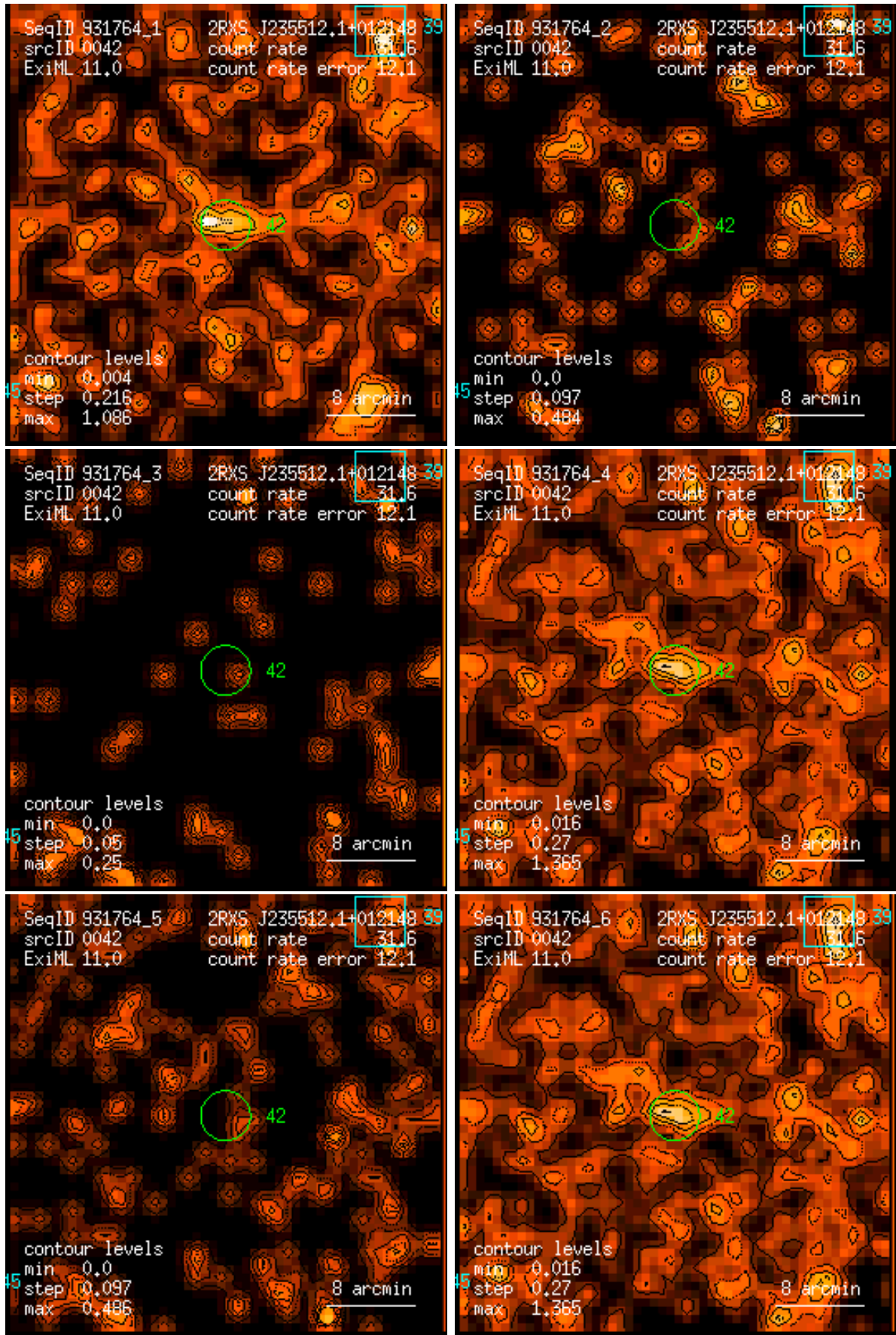
Figure 42: RASS 931764: detection 0042: band rate images, Gaussian filter: (1) PSPC channels 11 – 41, (2) 52 – 90, (3) 91 – 201, (4) 11 – 235, (5) 52 – 201, (6) 11 – 201. Broad band rates in counts/ks. Band rate contour levels in counts/ks/arcmin 2 .
