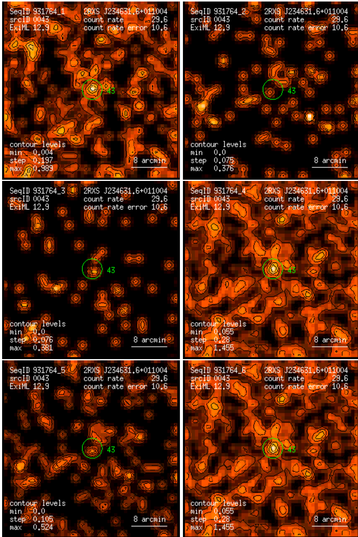
Figure 43: RASS 931764: detection 0043: band rate images, Gaussian filter: (1) PSPC channels 11 – 41, (2) 52 – 90, (3) 91 – 201, (4) 11 – 235, (5) 52 – 201, (6) 11 – 201. Broad band rates in counts/ks. Band rate contour levels in counts/ks/arcmin 2 .
