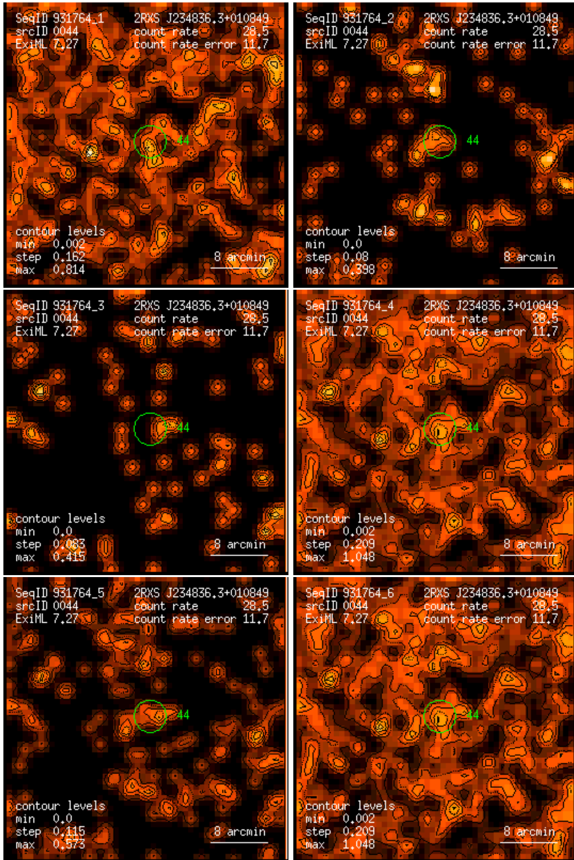
Figure 44: RASS 931764: detection 0044: band rate images, Gaussian filter: (1) PSPC channels 11 – 41, (2) 52 – 90, (3) 91 – 201, (4) 11 – 235, (5) 52 – 201, (6) 11 – 201. Broad band rates in counts/ks. Band rate contour levels in counts/ks/arcmin 2 .
