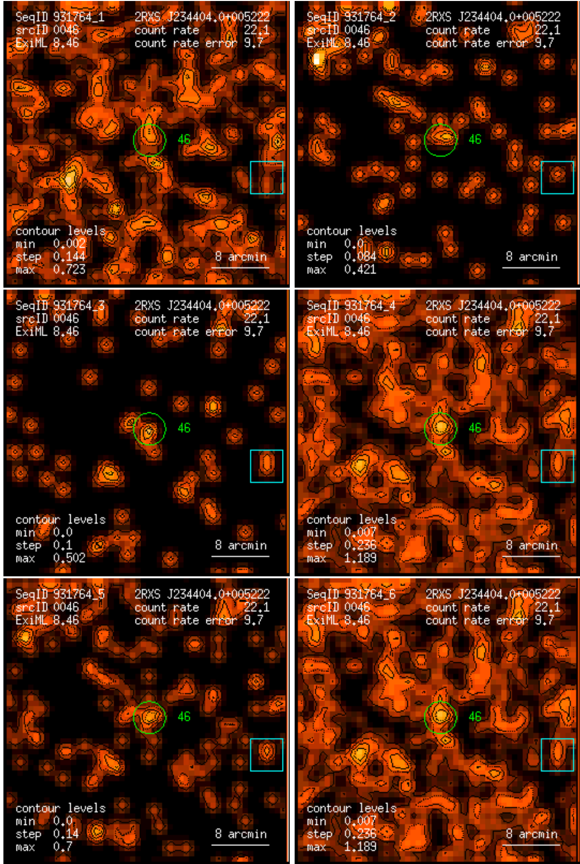
Figure 46: RASS 931764: detection 0046: band rate images, Gaussian filter: (1) PSPC channels 11 – 41, (2) 52 – 90, (3) 91 – 201, (4) 11 – 235, (5) 52 – 201, (6) 11 – 201. Broad band rates in counts/ks. Band rate contour levels in counts/ks/arcmin 2 .
