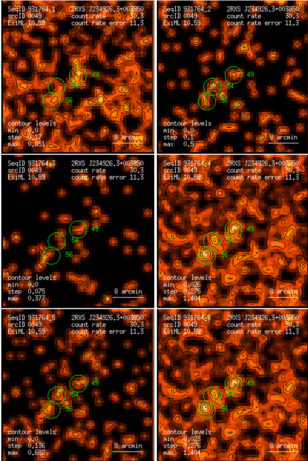
Figure 49: RASS 931764: detection 0049: band rate images, Gaussian filter: (1) PSPC channels 11 – 41, (2) 52 – 90, (3) 91 – 201, (4) 11 – 235, (5) 52 – 201, (6) 11 – 201. Broad band rates in counts/ks. Band rate contour levels in counts/ks/arcmin 2 .
