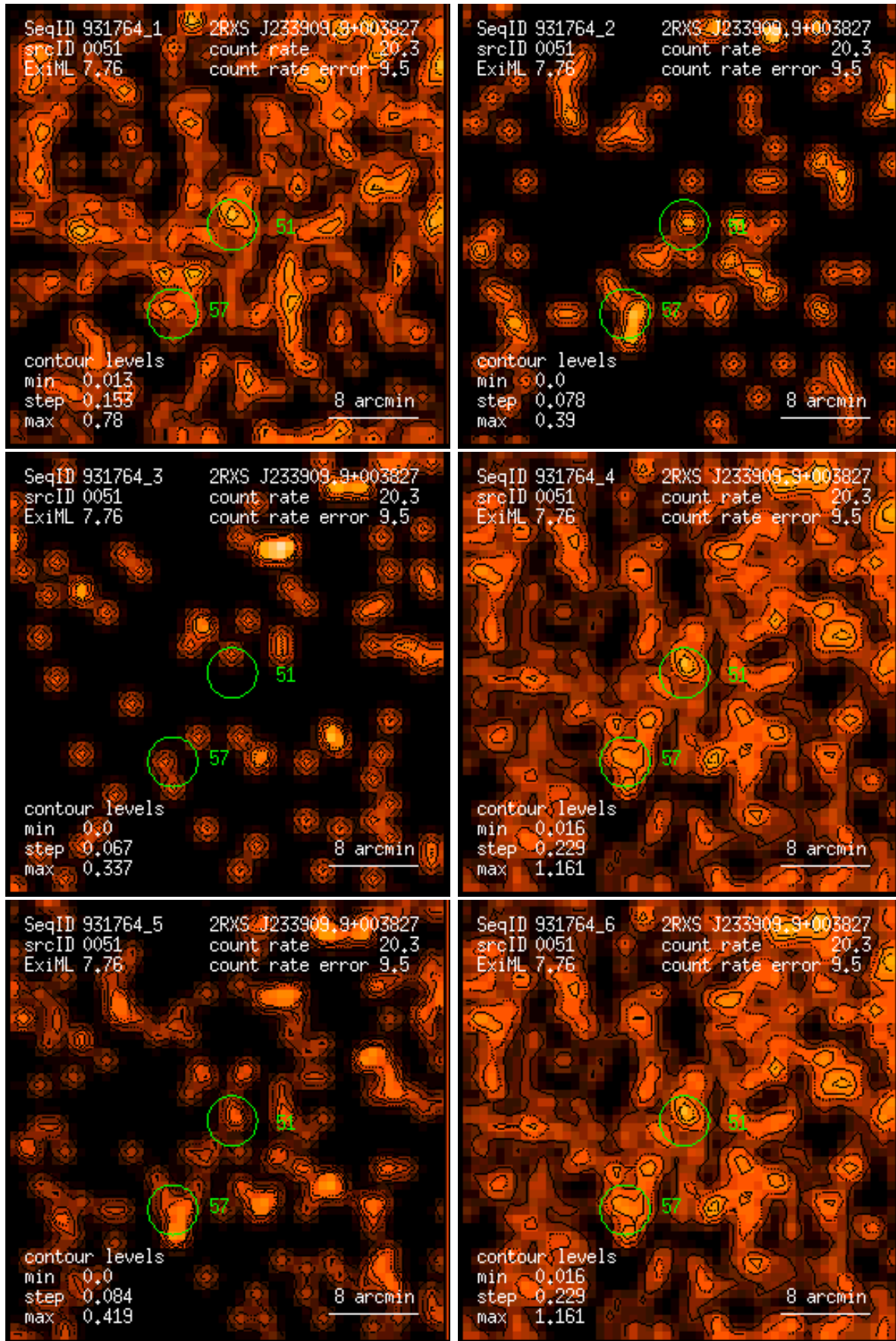
Figure 51: RASS 931764: detection 0051: band rate images, Gaussian filter: (1) PSPC channels 11 – 41, (2) 52 – 90, (3) 91 – 201, (4) 11 – 235, (5) 52 – 201, (6) 11 – 201. Broad band rates in counts/ks. Band rate contour levels in counts/ks/arcmin 2 .
