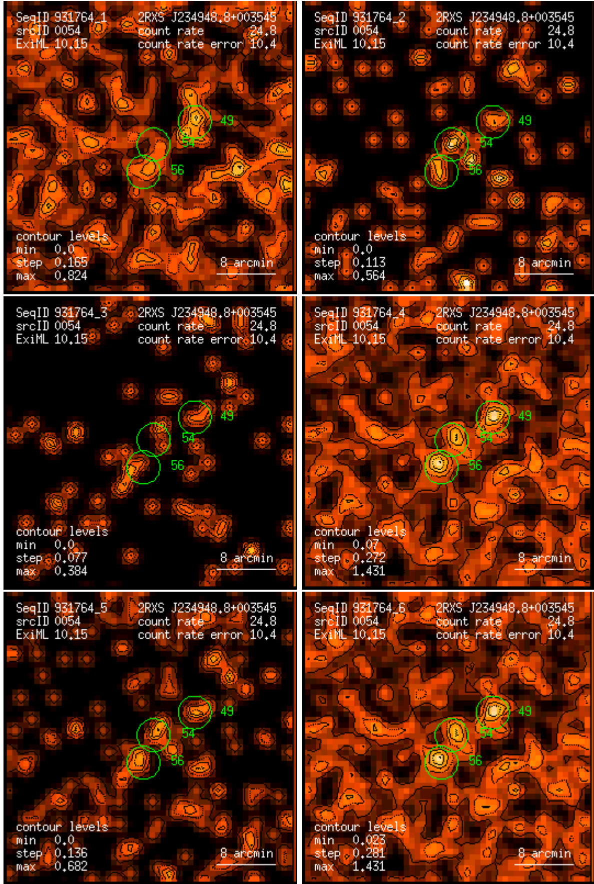
Figure 54: RASS 931764: detection 0054: band rate images, Gaussian filter: (1) PSPC channels 11 – 41, (2) 52 – 90, (3) 91 – 201, (4) 11 – 235, (5) 52 – 201, (6) 11 – 201. Broad band rates in counts/ks. Band rate contour levels in counts/ks/arcmin 2 .
