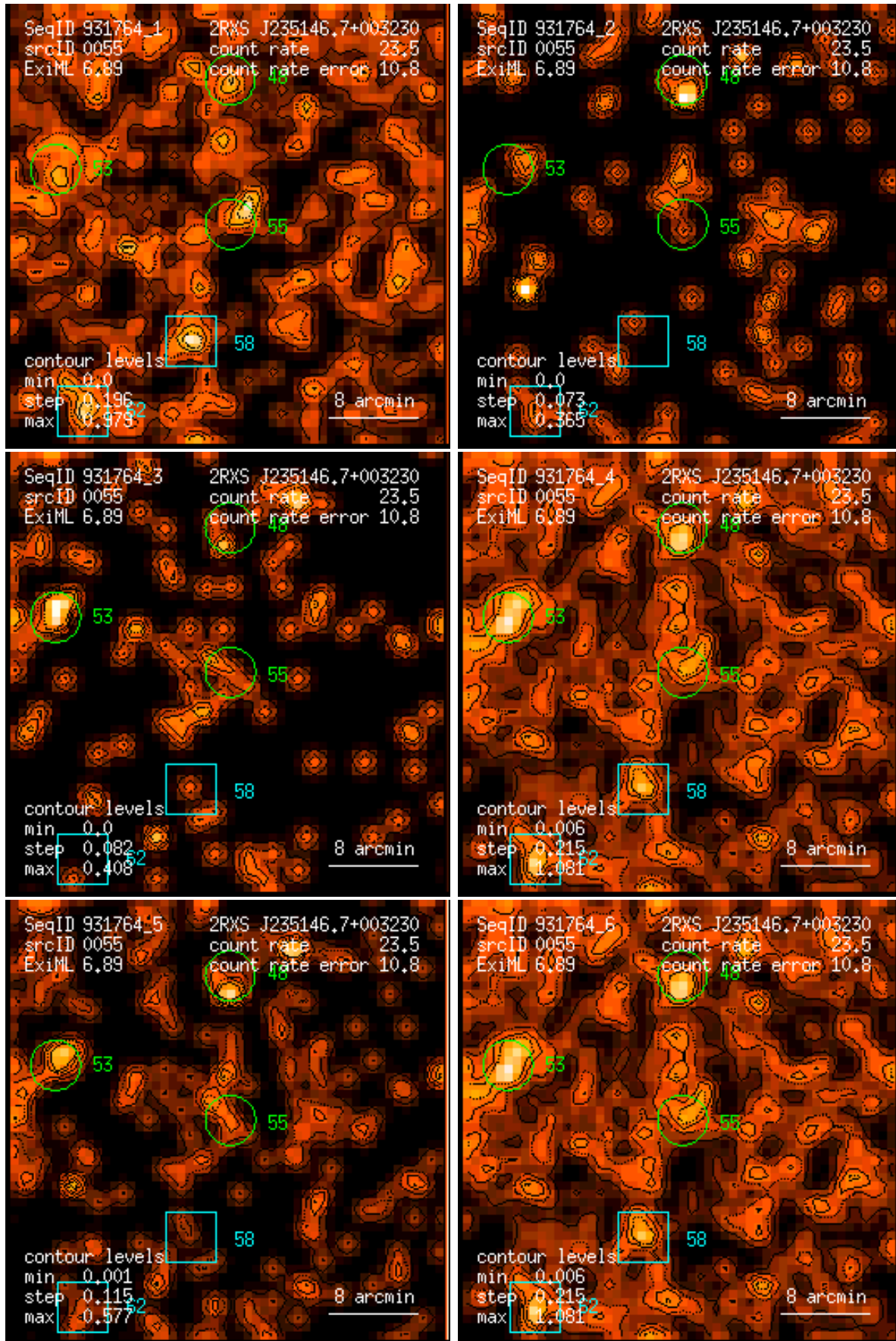
Figure 55: RASS 931764: detection 0055: band rate images, Gaussian filter: (1) PSPC channels 11 – 41, (2) 52 – 90, (3) 91 – 201, (4) 11 – 235, (5) 52 – 201, (6) 11 – 201. Broad band rates in counts/ks. Band rate contour levels in counts/ks/arcmin 2 .
