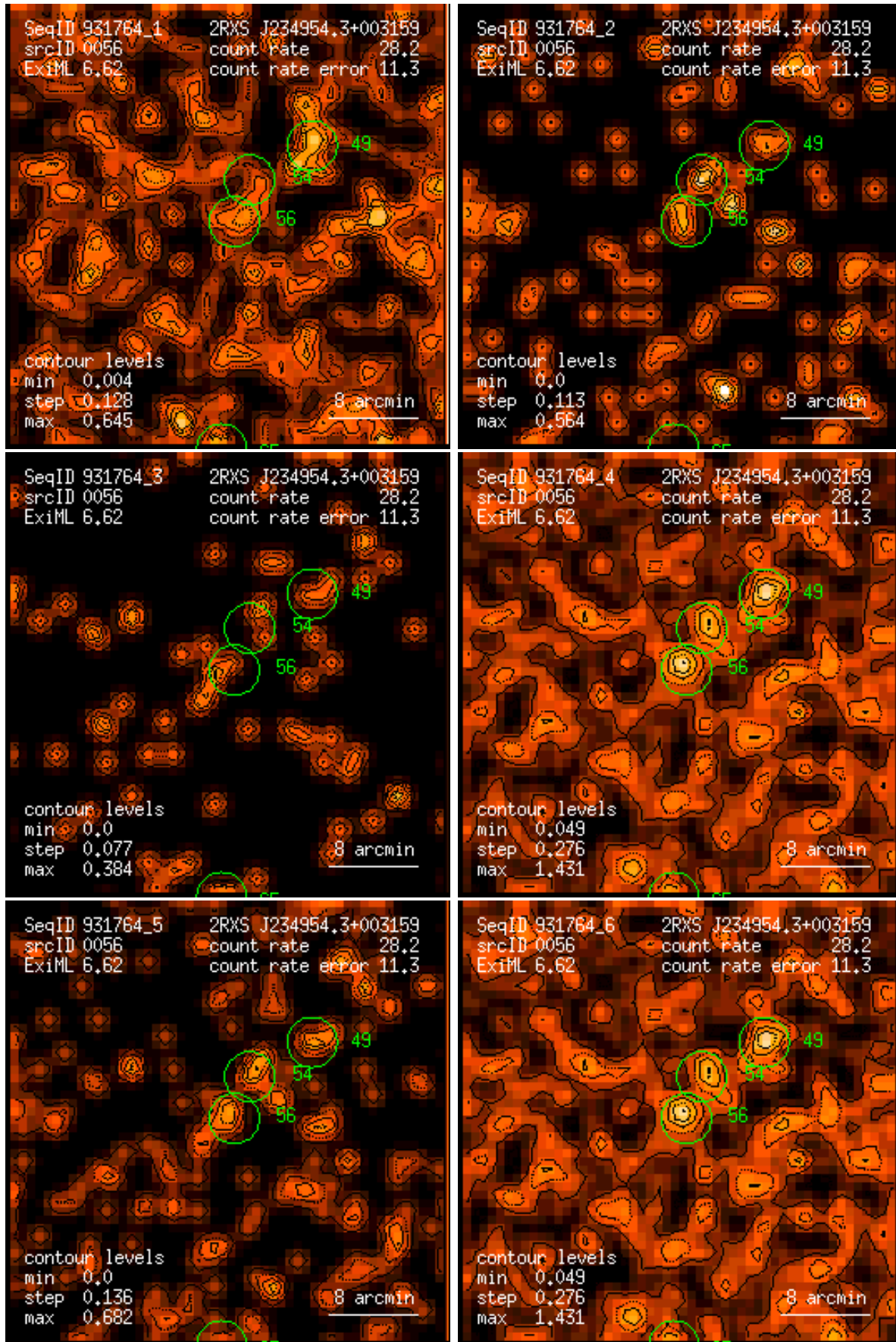
Figure 56: RASS 931764: detection 0056: band rate images, Gaussian filter: (1) PSPC channels 11 – 41, (2) 52 – 90, (3) 91 – 201, (4) 11 – 235, (5) 52 – 201, (6) 11 – 201. Broad band rates in counts/ks. Band rate contour levels in counts/ks/arcmin 2 .
