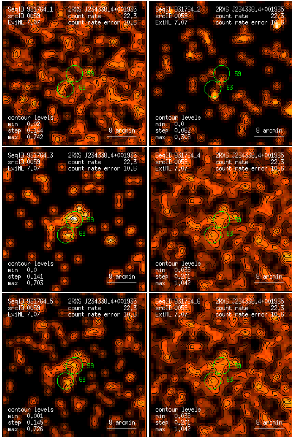
Figure 59: RASS 931764: detection 0059: band rate images, Gaussian filter: (1) PSPC channels 11 – 41, (2) 52 – 90, (3) 91 – 201, (4) 11 – 235, (5) 52 – 201, (6) 11 – 201. Broad band rates in counts/ks. Band rate contour levels in counts/ks/arcmin 2 .
