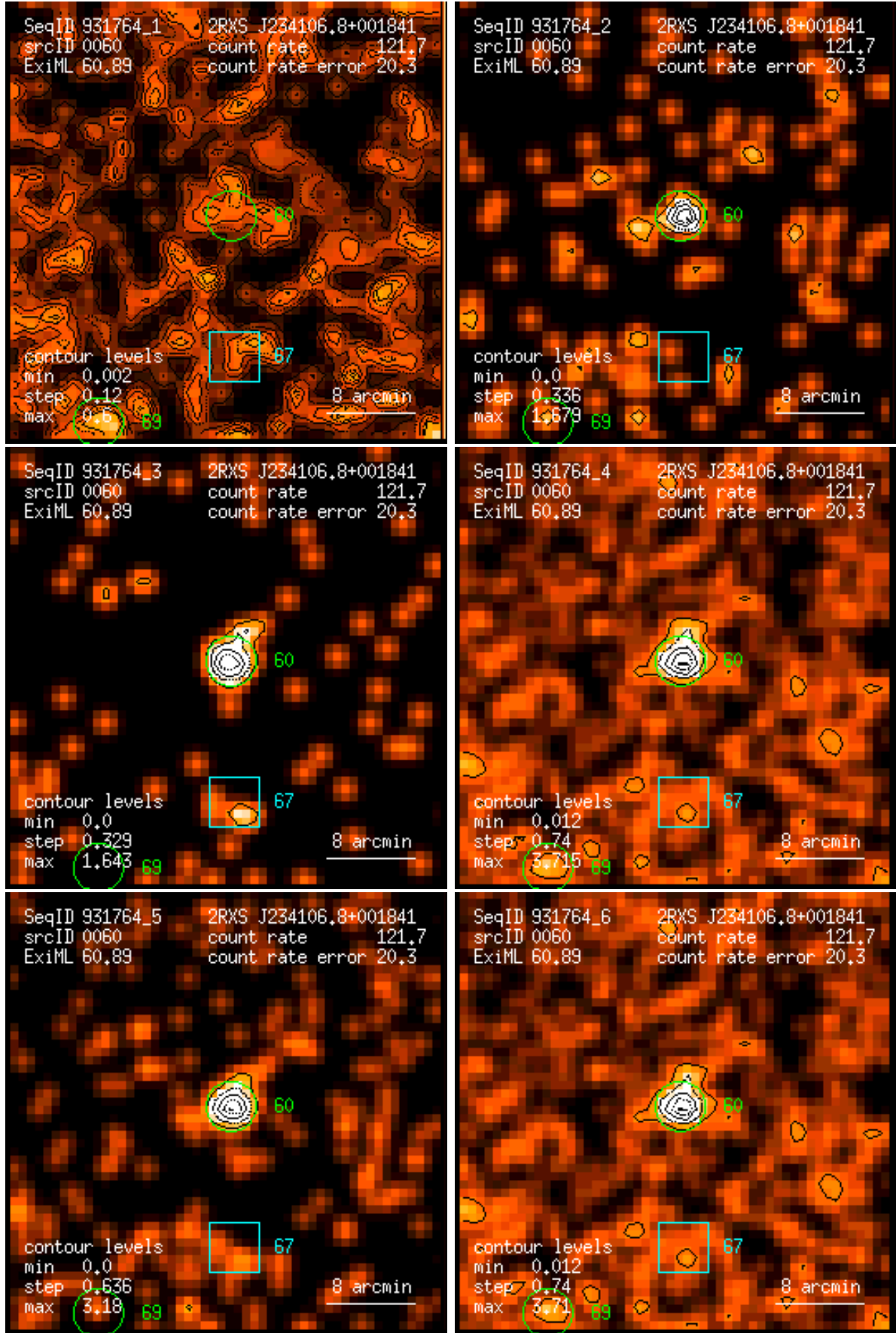
Figure 60: RASS 931764: detection 0060: band rate images, Gaussian filter: (1) PSPC channels 11 – 41, (2) 52 – 90, (3) 91 – 201, (4) 11 – 235, (5) 52 – 201, (6) 11 – 201. Broad band rates in counts/ks. Band rate contour levels in counts/ks/arcmin 2 .
