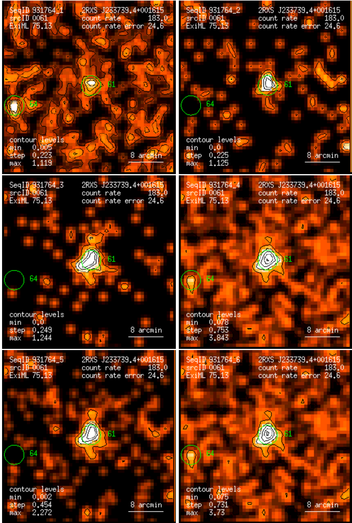
Figure 61: RASS 931764: detection 0061: band rate images, Gaussian filter: (1) PSPC channels 11 – 41, (2) 52 – 90, (3) 91 – 201, (4) 11 – 235, (5) 52 – 201, (6) 11 – 201. Broad band rates in counts/ks. Band rate contour levels in counts/ks/arcmin 2 .
