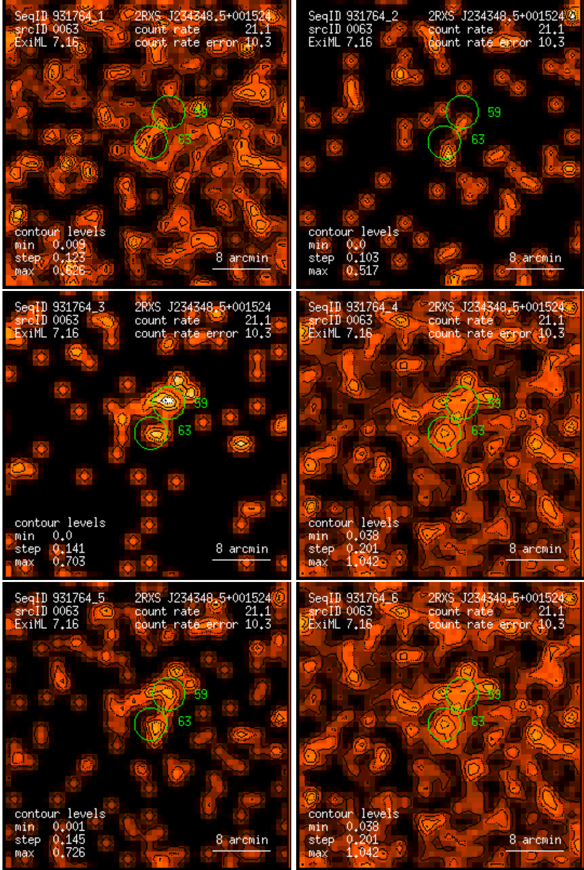
Figure 63: RASS 931764: detection 0063: band rate images, Gaussian filter: (1) PSPC channels 11 – 41, (2) 52 – 90, (3) 91 – 201, (4) 11 – 235, (5) 52 – 201, (6) 11 – 201. Broad band rates in counts/ks. Band rate contour levels in counts/ks/arcmin 2 .
