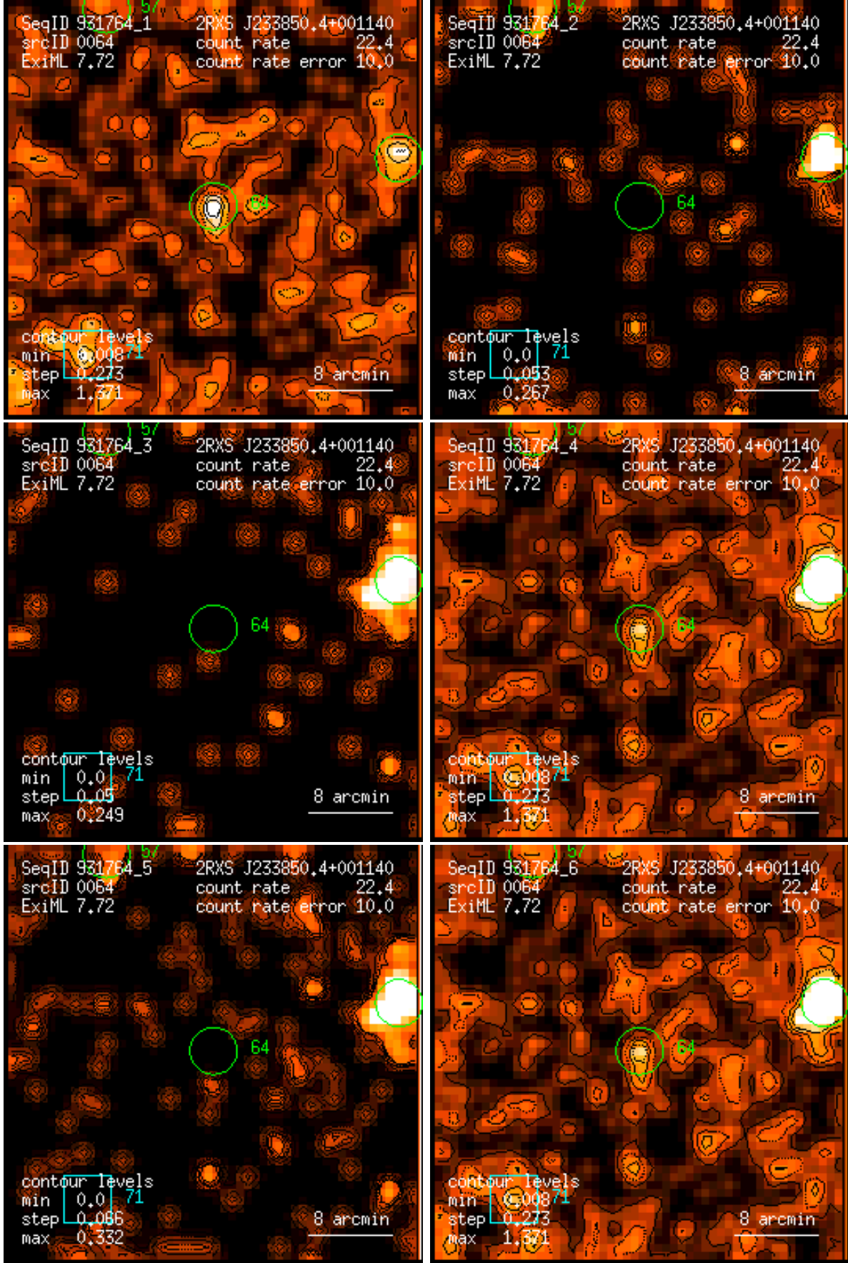
Figure 64: RASS 931764: detection 0064: band rate images, Gaussian filter: (1) PSPC channels 11 – 41, (2) 52 – 90, (3) 91 – 201, (4) 11 – 235, (5) 52 – 201, (6) 11 – 201. Broad band rates in counts/ks. Band rate contour levels in counts/ks/arcmin 2 .
