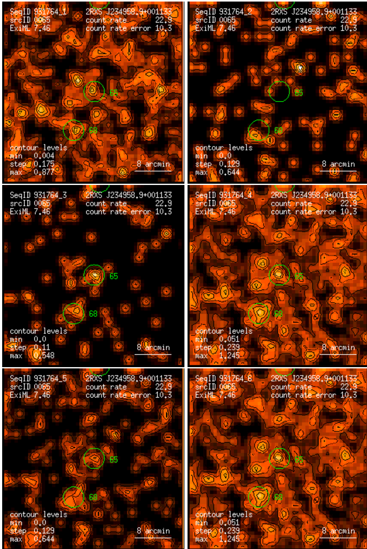
Figure 65: RASS 931764: detection 0065: band rate images, Gaussian filter: (1) PSPC channels 11 – 41, (2) 52 – 90, (3) 91 – 201, (4) 11 – 235, (5) 52 – 201, (6) 11 – 201. Broad band rates in counts/ks. Band rate contour levels in counts/ks/arcmin 2 .
