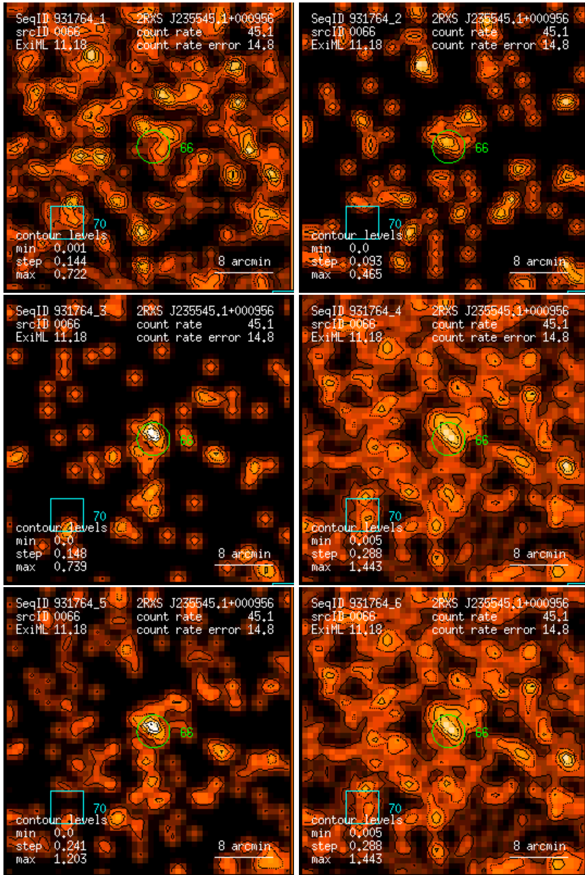
Figure 66: RASS 931764: detection 0066: band rate images, Gaussian filter: (1) PSPC channels 11 – 41, (2) 52 – 90, (3) 91 – 201, (4) 11 – 235, (5) 52 – 201, (6) 11 – 201. Broad band rates in counts/ks. Band rate contour levels in counts/ks/arcmin 2 .
