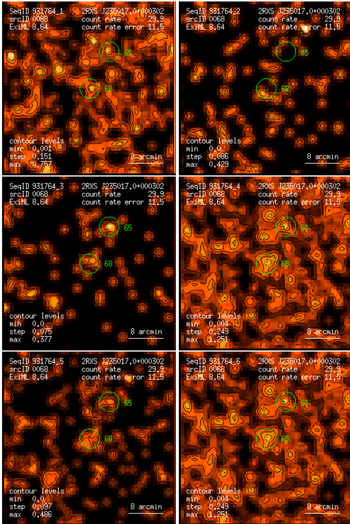
Figure 68: RASS 931764: detection 0068: band rate images, Gaussian filter: (1) PSPC channels 11 – 41, (2) 52 – 90, (3) 91 – 201, (4) 11 – 235, (5) 52 – 201, (6) 11 – 201. Broad band rates in counts/ks. Band rate contour levels in counts/ks/arcmin 2 .
