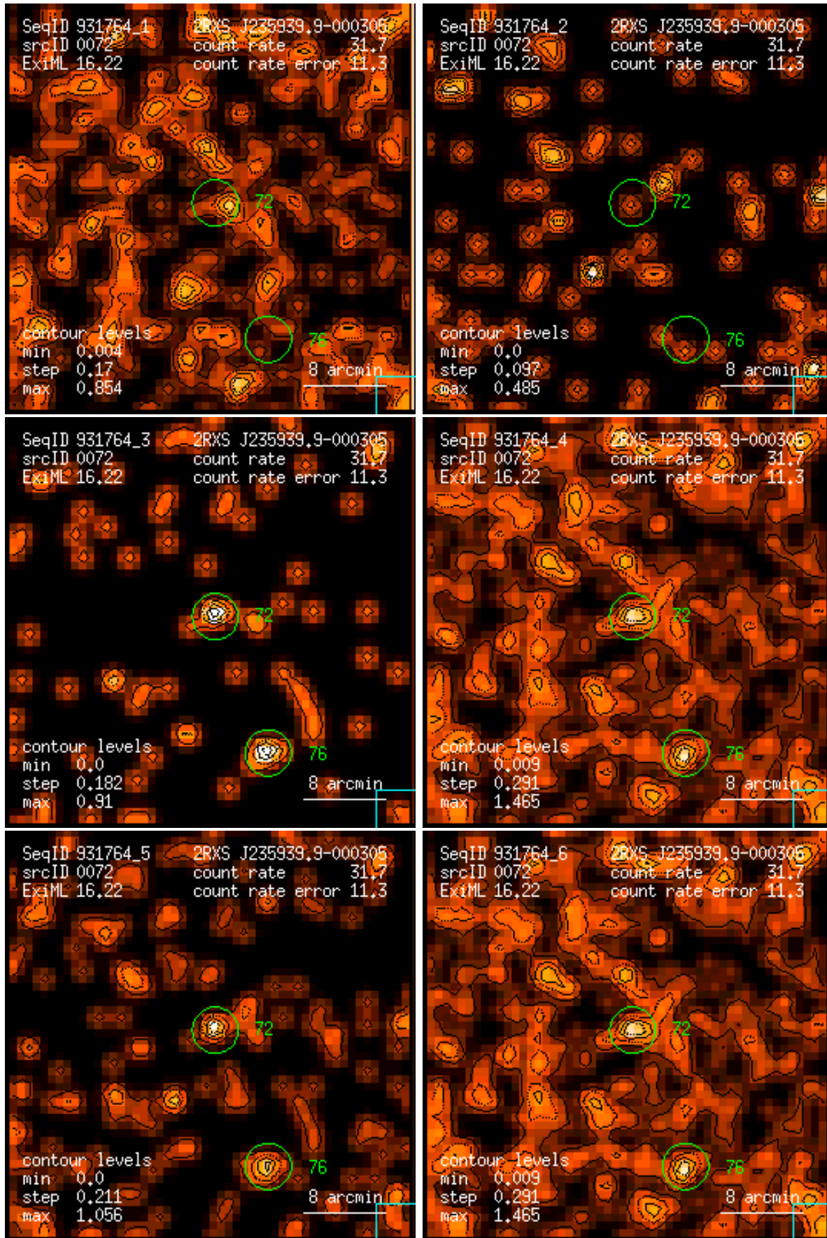
Figure 72: RASS 931764: detection 0072: band rate images, Gaussian filter: (1) PSPC channels 11 – 41, (2) 52 – 90, (3) 91 – 201, (4) 11 – 235, (5) 52 – 201, (6) 11 – 201. Broad band rates in counts/ks. Band rate contour levels in counts/ks/arcmin 2 .
