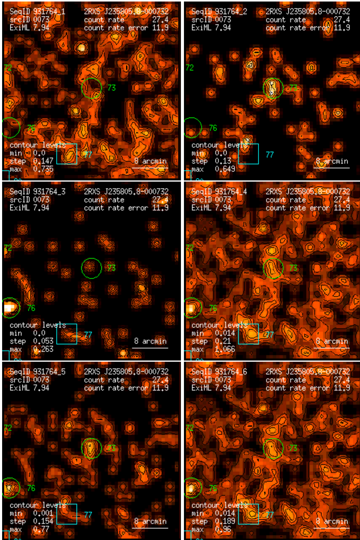
Figure 73: RASS 931764: detection 0073: band rate images, Gaussian filter: (1) PSPC channels 11 – 41, (2) 52 – 90, (3) 91 – 201, (4) 11 – 235, (5) 52 – 201, (6) 11 – 201. Broad band rates in counts/ks. Band rate contour levels in counts/ks/arcmin 2 .
