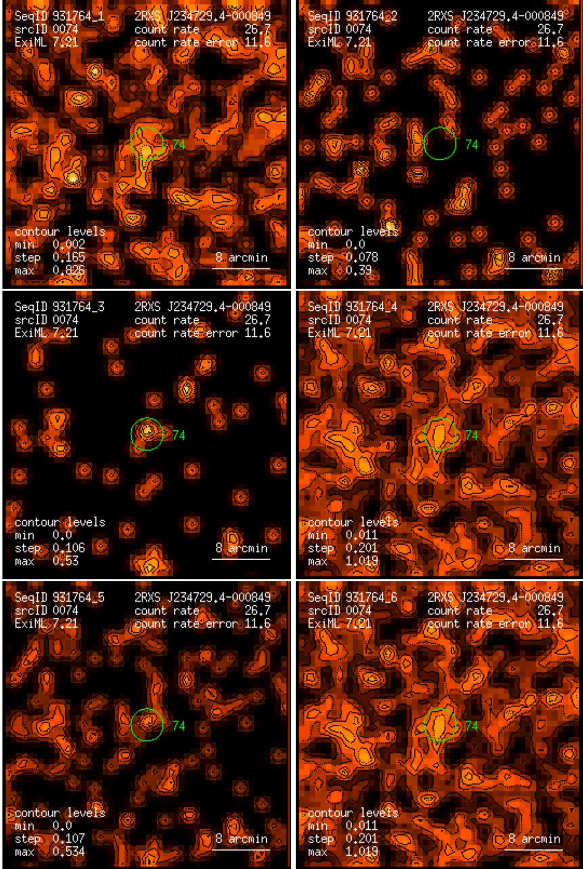
Figure 74: RASS 931764: detection 0074: band rate images, Gaussian filter: (1) PSPC channels 11 – 41, (2) 52 – 90, (3) 91 – 201, (4) 11 – 235, (5) 52 – 201, (6) 11 – 201. Broad band rates in counts/ks. Band rate contour levels in counts/ks/arcmin 2 .
