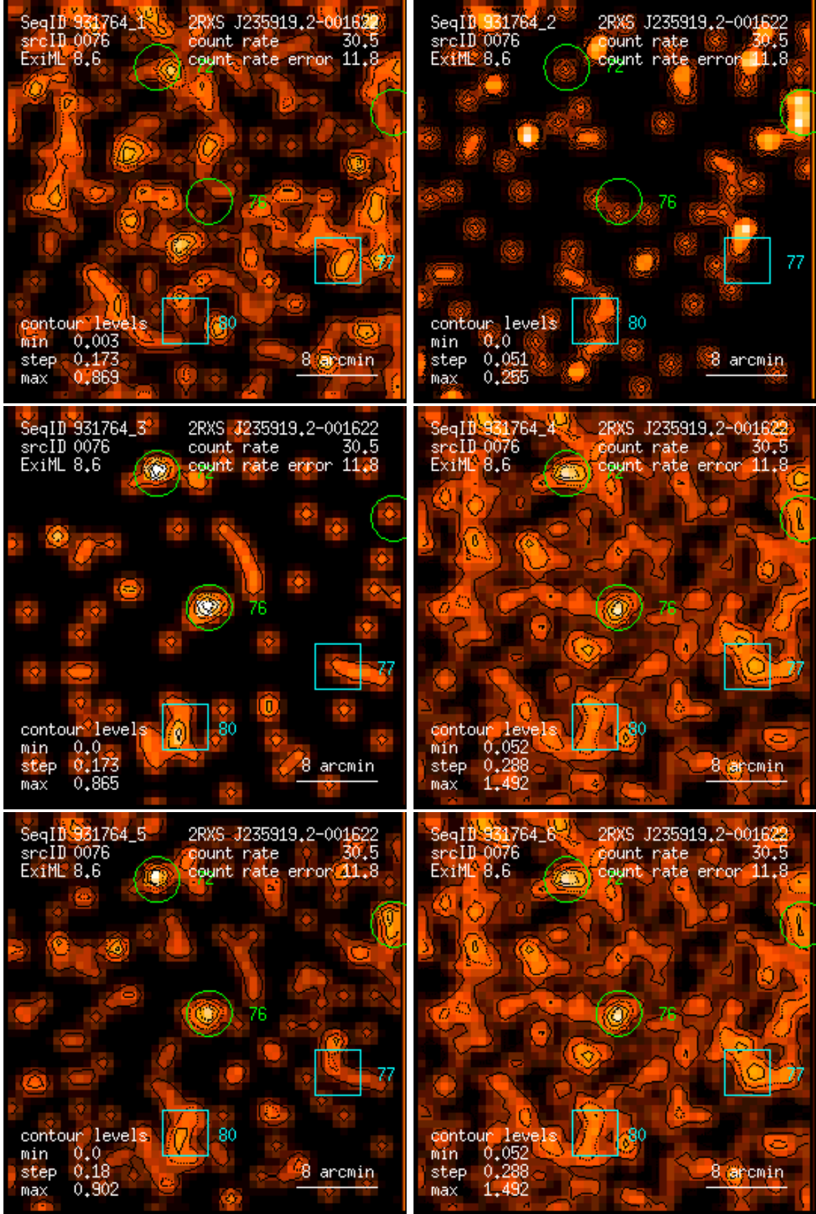
Figure 76: RASS 931764: detection 0076: band rate images, Gaussian filter: (1) PSPC channels 11 – 41, (2) 52 – 90, (3) 91 – 201, (4) 11 – 235, (5) 52 – 201, (6) 11 – 201. Broad band rates in counts/ks. Band rate contour levels in counts/ks/arcmin 2 .
