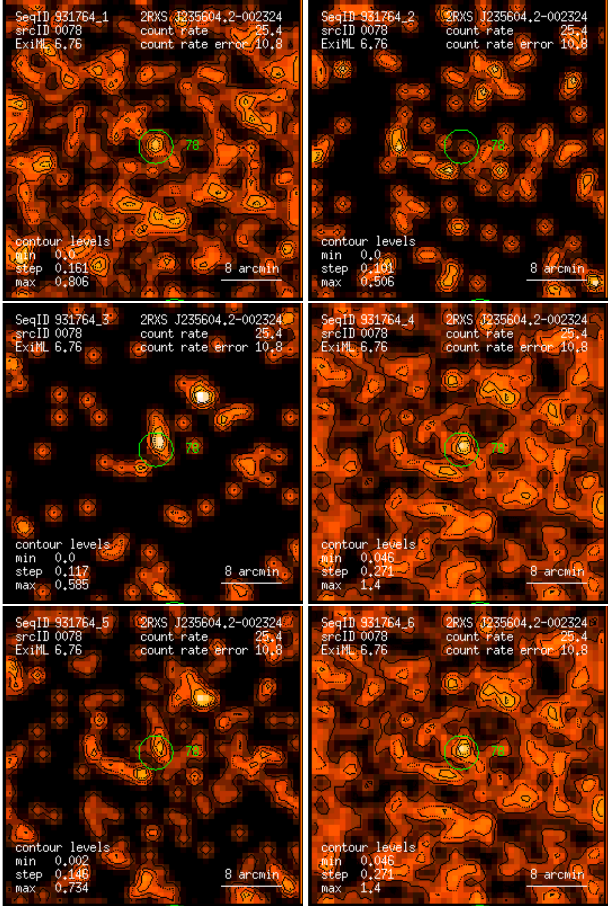
Figure 78: RASS 931764: detection 0078: band rate images, Gaussian filter: (1) PSPC channels 11 – 41, (2) 52 – 90, (3) 91 – 201, (4) 11 – 235, (5) 52 – 201, (6) 11 – 201. Broad band rates in counts/ks. Band rate contour levels in counts/ks/arcmin 2 .
