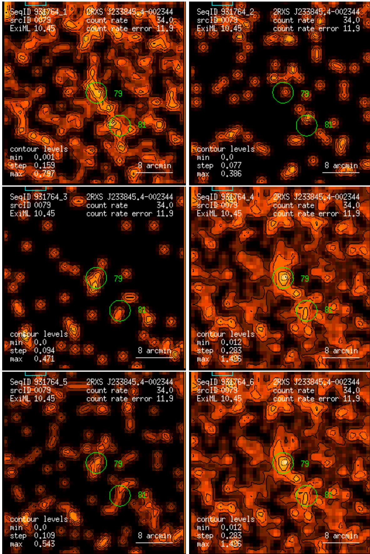
Figure 79: RASS 931764: detection 0079: band rate images, Gaussian filter: (1) PSPC channels 11 – 41, (2) 52 – 90, (3) 91 – 201, (4) 11 – 235, (5) 52 – 201, (6) 11 – 201. Broad band rates in counts/ks. Band rate contour levels in counts/ks/arcmin 2 .
