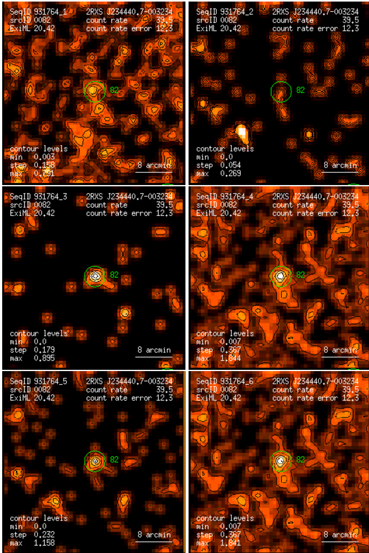
Figure 82: RASS 931764: detection 0082: band rate images, Gaussian filter: (1) PSPC channels 11 – 41, (2) 52 – 90, (3) 91 – 201, (4) 11 – 235, (5) 52 – 201, (6) 11 – 201. Broad band rates in counts/ks. Band rate contour levels in counts/ks/arcmin 2 .
