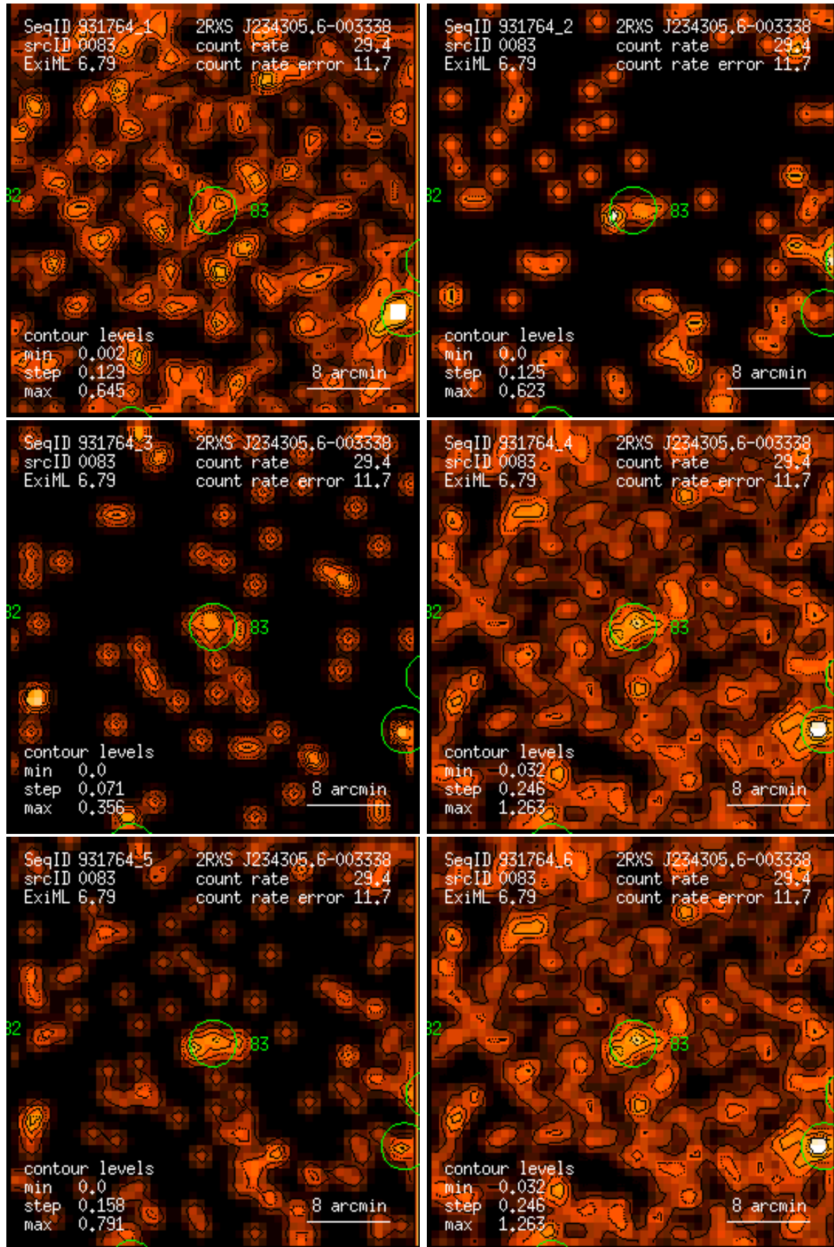
Figure 83: RASS 931764: detection 0083: band rate images, Gaussian filter: (1) PSPC channels 11 – 41, (2) 52 – 90, (3) 91 – 201, (4) 11 – 235, (5) 52 – 201, (6) 11 – 201. Broad band rates in counts/ks. Band rate contour levels in counts/ks/arcmin 2 .
