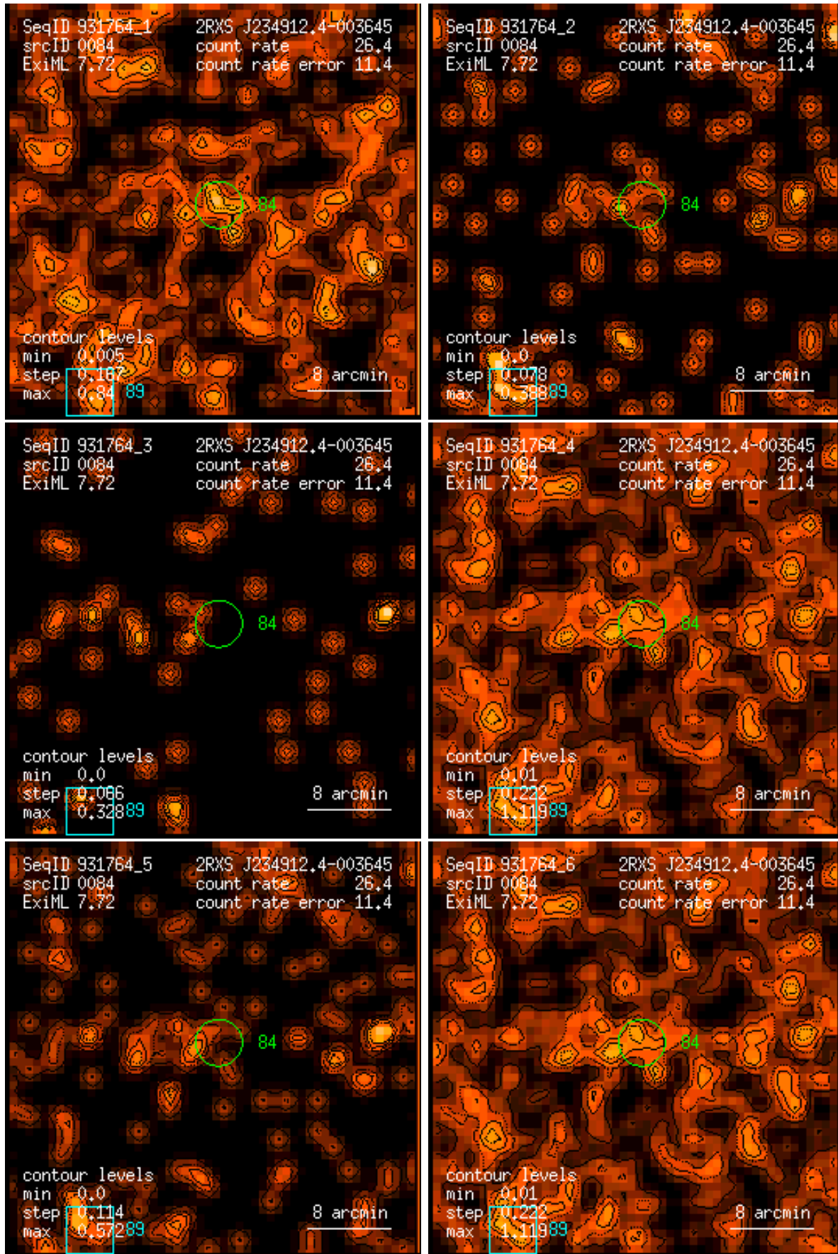
Figure 84: RASS 931764: detection 0084: band rate images, Gaussian filter: (1) PSPC channels 11 – 41, (2) 52 – 90, (3) 91 – 201, (4) 11 – 235, (5) 52 – 201, (6) 11 – 201. Broad band rates in counts/ks. Band rate contour levels in counts/ks/arcmin 2 .
