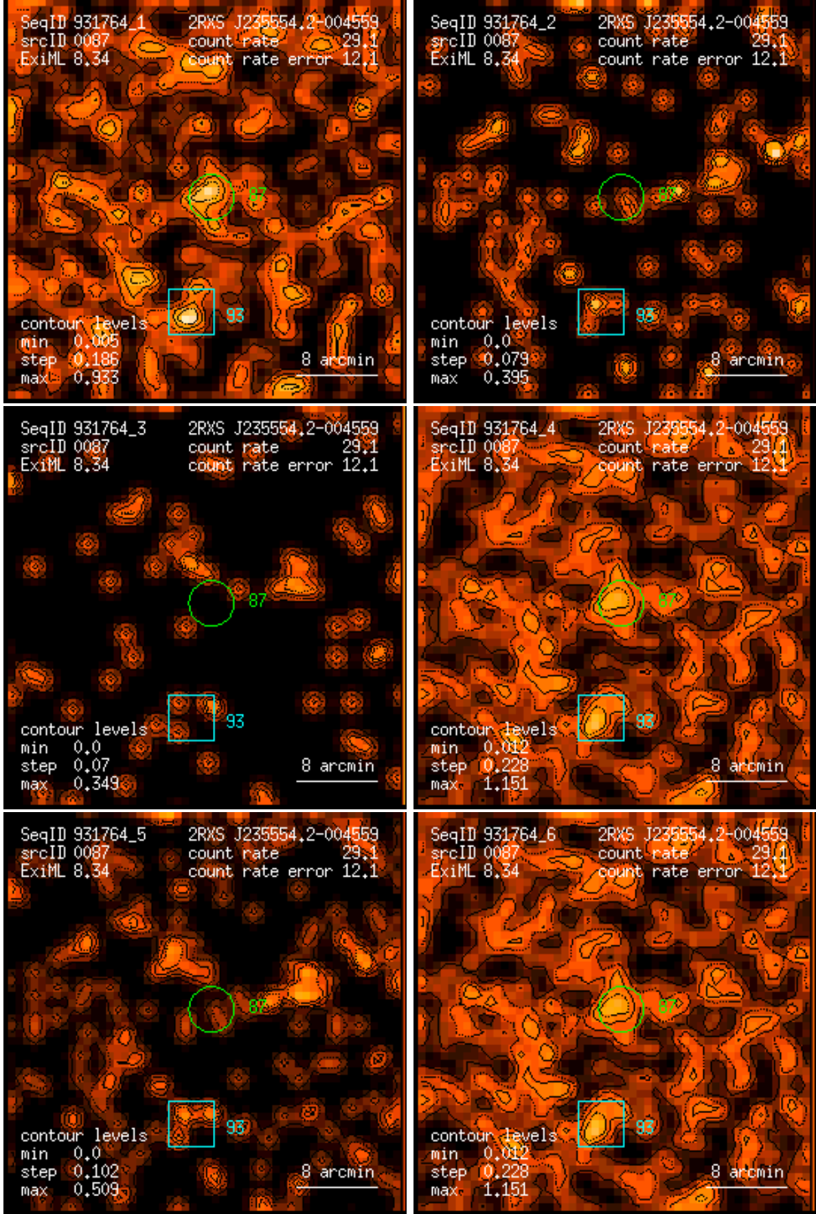
Figure 87: RASS 931764: detection 0087: band rate images, Gaussian filter: (1) PSPC channels 11 – 41, (2) 52 – 90, (3) 91 – 201, (4) 11 – 235, (5) 52 – 201, (6) 11 – 201. Broad band rates in counts/ks. Band rate contour levels in counts/ks/arcmin 2 .
