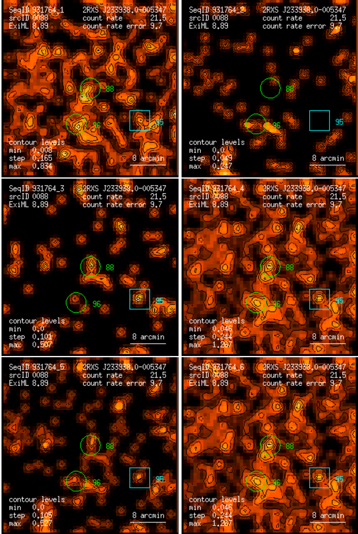
Figure 88: RASS 931764: detection 0088: band rate images, Gaussian filter: (1) PSPC channels 11 – 41, (2) 52 – 90, (3) 91 – 201, (4) 11 – 235, (5) 52 – 201, (6) 11 – 201. Broad band rates in counts/ks. Band rate contour levels in counts/ks/arcmin 2 .
