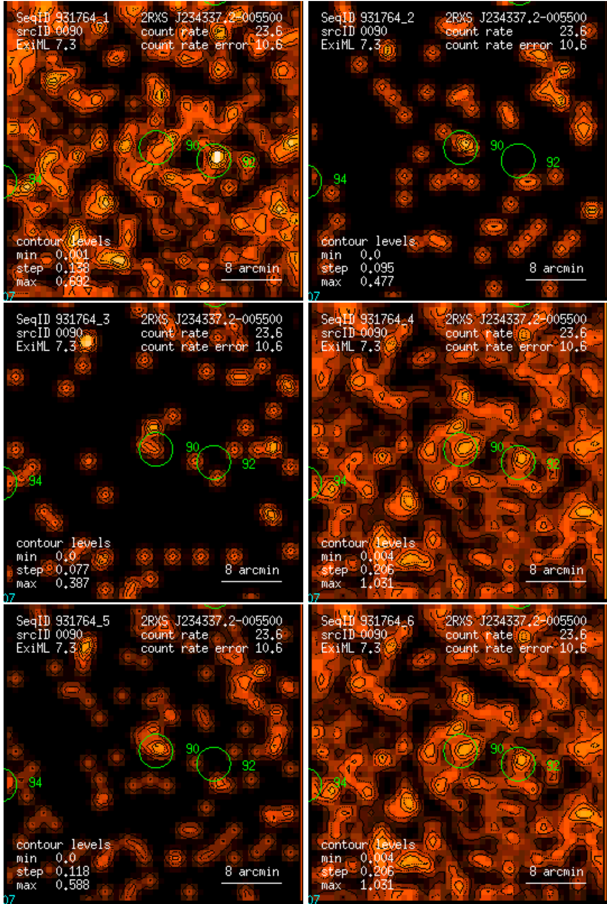
Figure 90: RASS 931764: detection 0090: band rate images, Gaussian filter: (1) PSPC channels 11 – 41, (2) 52 – 90, (3) 91 – 201, (4) 11 – 235, (5) 52 – 201, (6) 11 – 201. Broad band rates in counts/ks. Band rate contour levels in counts/ks/arcmin 2 .
