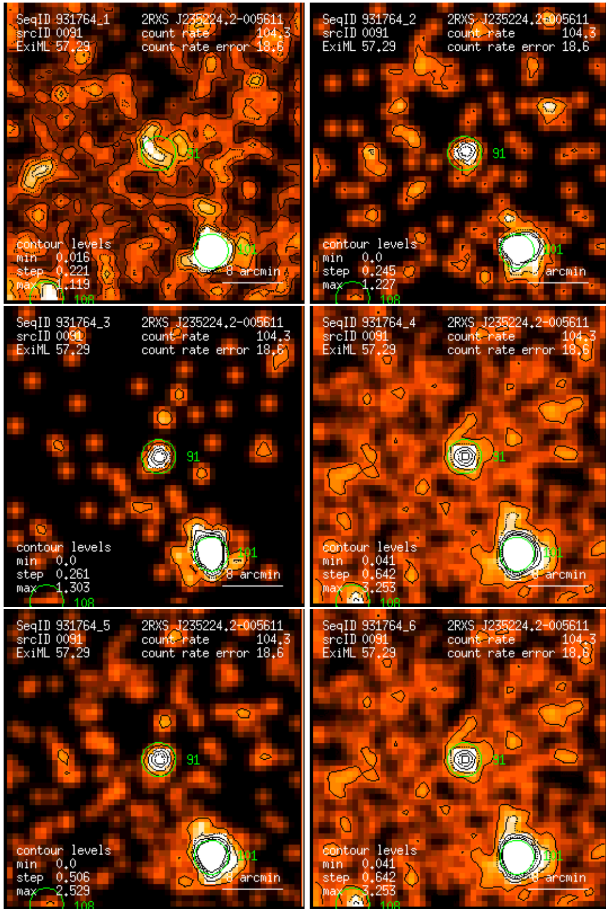
Figure 91: RASS 931764: detection 0091: band rate images, Gaussian filter: (1) PSPC channels 11 – 41, (2) 52 – 90, (3) 91 – 201, (4) 11 – 235, (5) 52 – 201, (6) 11 – 201. Broad band rates in counts/ks. Band rate contour levels in counts/ks/arcmin 2 .
