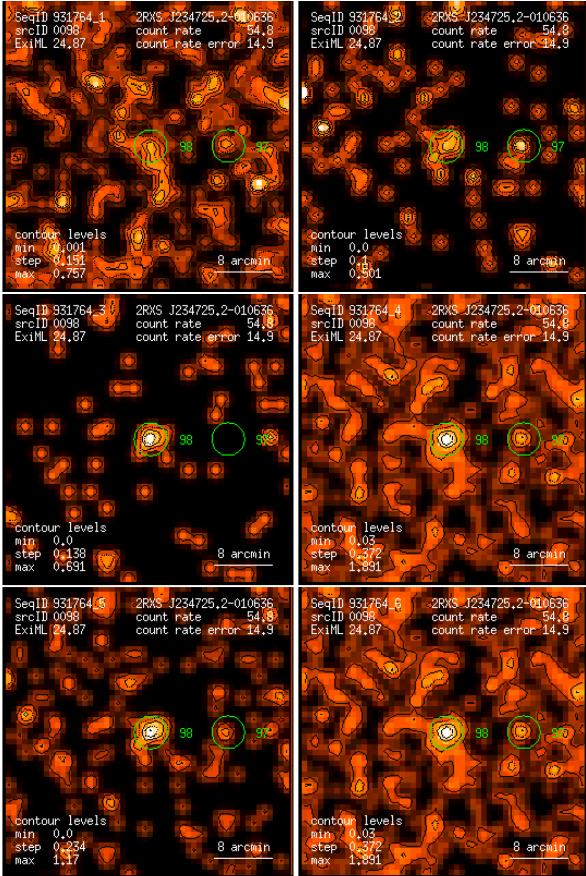
Figure 98: RASS 931764: detection 0098: band rate images, Gaussian filter: (1) PSPC channels 11 – 41, (2) 52 – 90, (3) 91 – 201, (4) 11 – 235, (5) 52 – 201, (6) 11 – 201. Broad band rates in counts/ks. Band rate contour levels in counts/ks/arcmin 2 .
