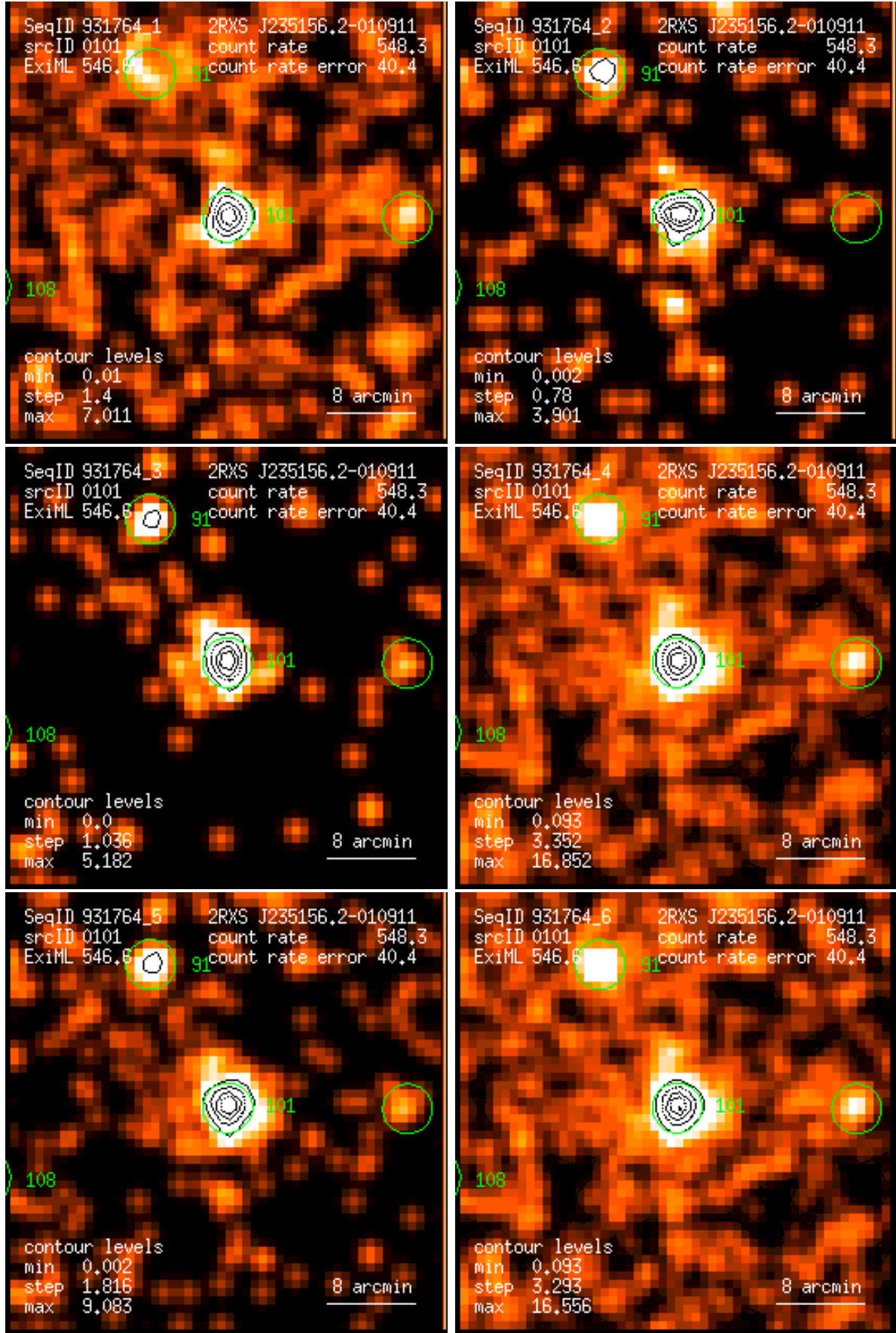
Figure 101: RASS 931764: detection 0101: band rate images, Gaussian filter: (1) PSPC channels 11 – 41, (2) 52 – 90, (3) 91 – 201, (4) 11 – 235, (5) 52 – 201, (6) 11 – 201. Broad band rates in counts/ks. Band rate contour levels in counts/ks/arcmin 2 .
