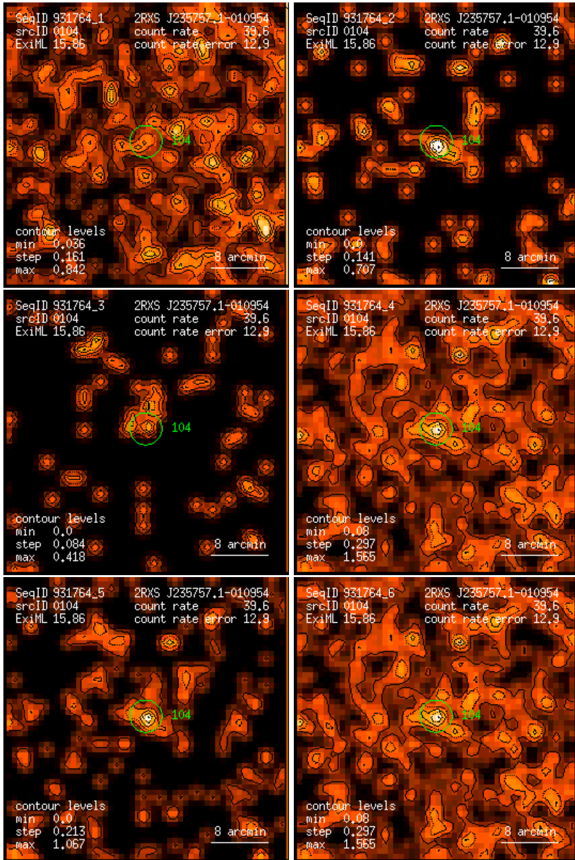
Figure 104: RASS 931764: detection 0104: band rate images, Gaussian filter: (1) PSPC channels 11 – 41, (2) 52 – 90, (3) 91 – 201, (4) 11 – 235, (5) 52 – 201, (6) 11 – 201. Broad band rates in counts/ks. Band rate contour levels in counts/ks/arcmin 2 .
