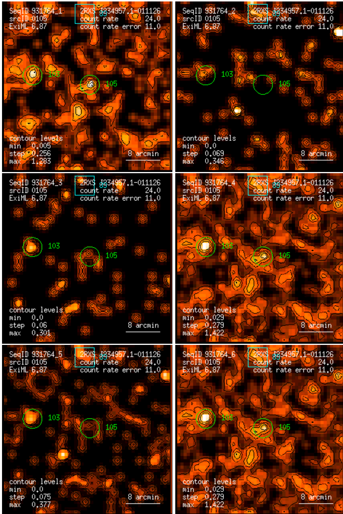
Figure 105: RASS 931764: detection 0105: band rate images, Gaussian filter: (1) PSPC channels 11 – 41, (2) 52 – 90, (3) 91 – 201, (4) 11 – 235, (5) 52 – 201, (6) 11 – 201. Broad band rates in counts/ks. Band rate contour levels in counts/ks/arcmin 2 .
