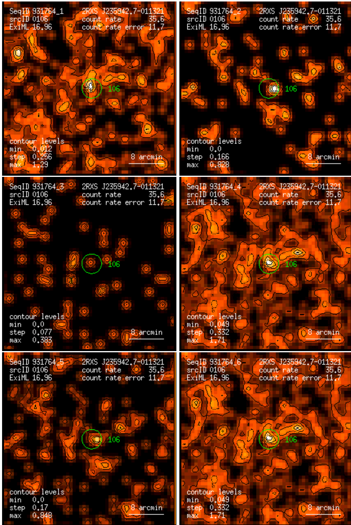
Figure 106: RASS 931764: detection 0106: band rate images, Gaussian filter: (1) PSPC channels 11 – 41, (2) 52 – 90, (3) 91 – 201, (4) 11 – 235, (5) 52 – 201, (6) 11 – 201. Broad band rates in counts/ks. Band rate contour levels in counts/ks/arcmin 2 .
