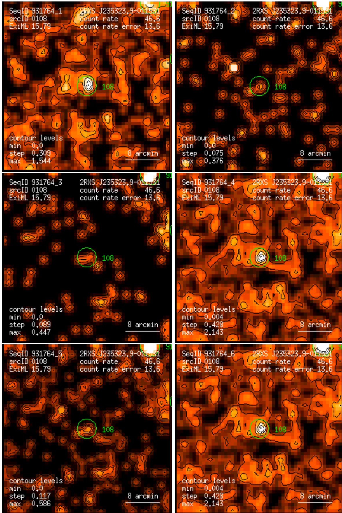
Figure 108: RASS 931764: detection 0108: band rate images, Gaussian filter: (1) PSPPC channels 11 – 41, (2) 52 – 90, (3) 91 – 201, (4) 11 – 235, (5) 52 – 201, (6) 11 – 201. Broad band rates in counts/ks. Band rate contour levels in counts/ks/arcmin 2 .
