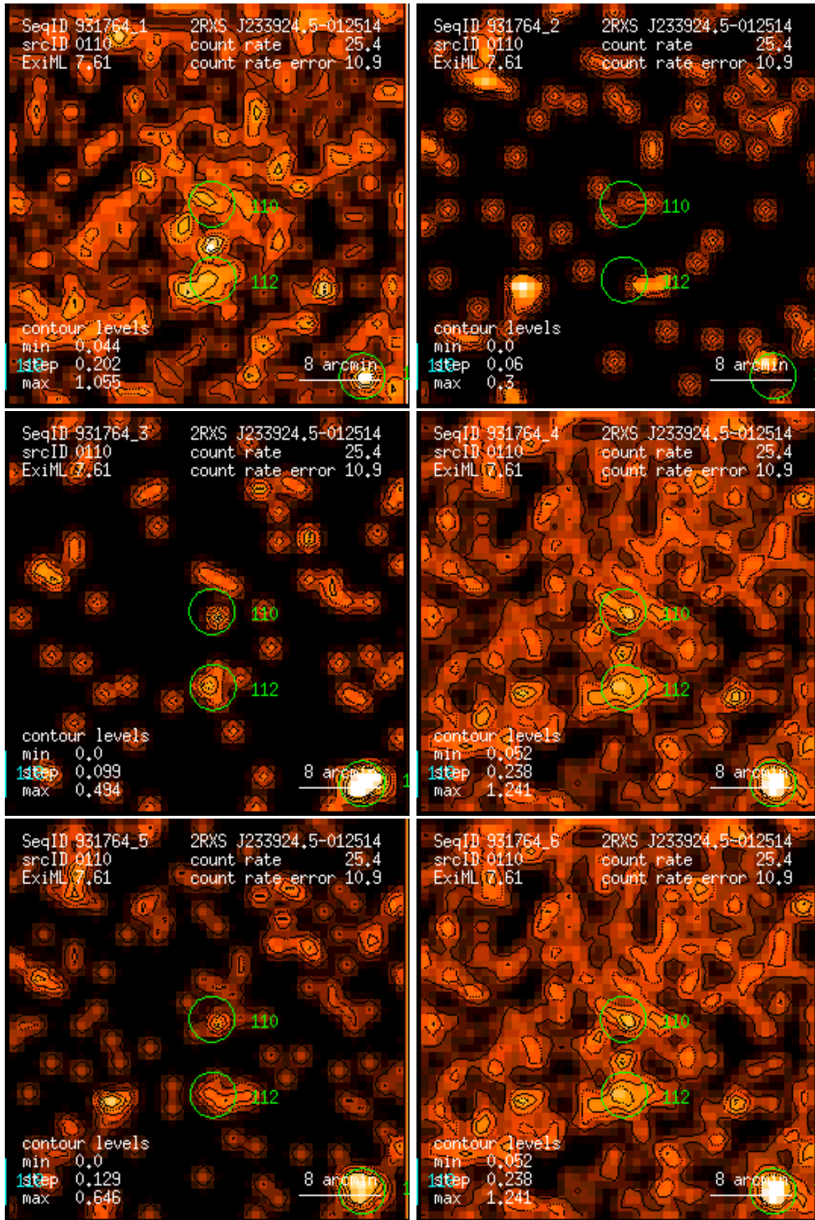
Figure 110: RASS 931764: detection 0110: band rate images, Gaussian filter: (1) PSPC channels 11 – 41, (2) 52 – 90, (3) 91 – 201, (4) 11 – 235, (5) 52 – 201, (6) 11 – 201. Broad band rates in counts/ks. Band rate contour levels in counts/ks/arcmin 2 .
