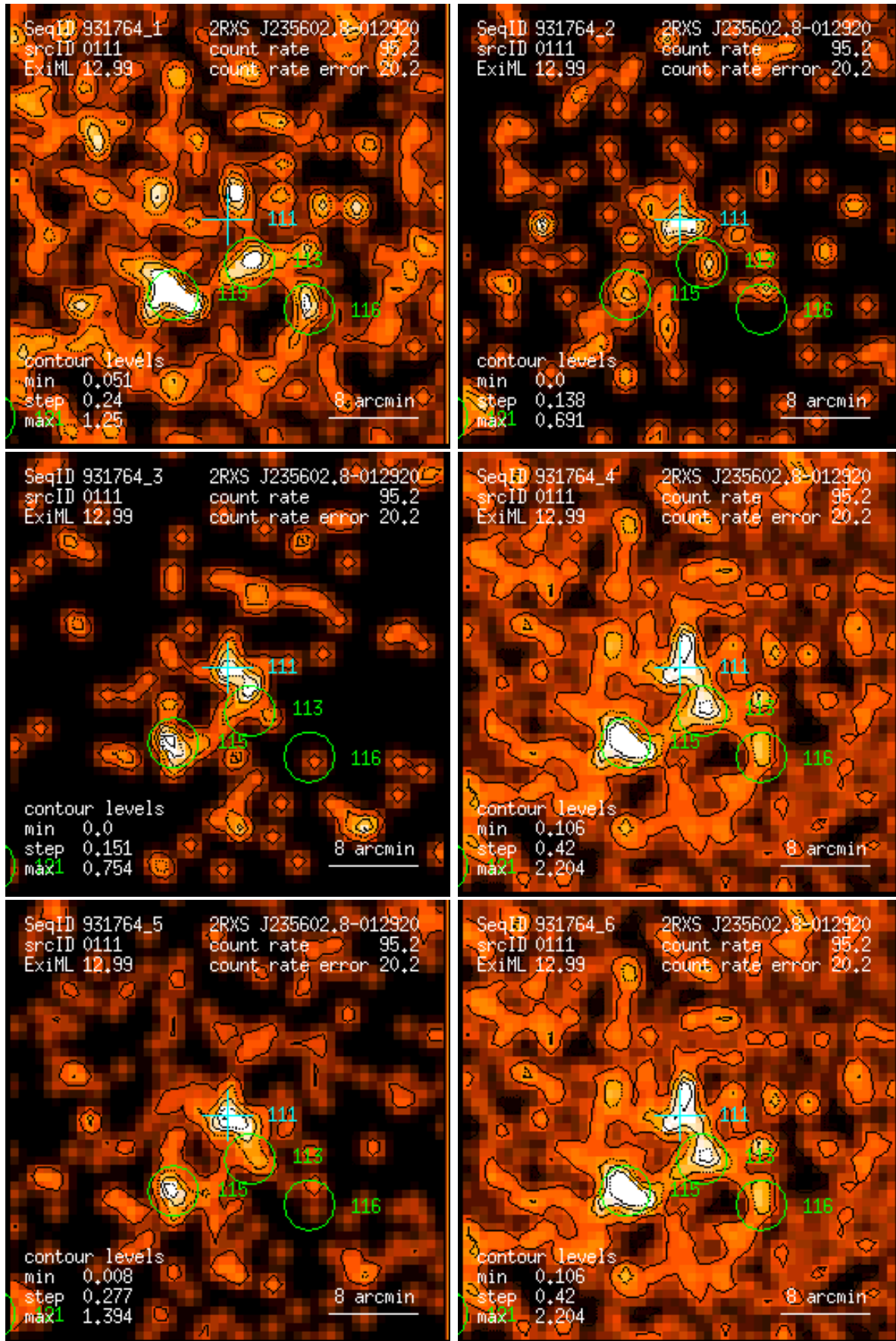
Figure 111: RASS 931764: detection 0111: band rate images, Gaussian filter: (1) PSPC channels 11 – 41, (2) 52 – 90, (3) 91 – 201, (4) 11 – 235, (5) 52 – 201, (6) 11 – 201. Broad band rates in counts/ks. Band rate contour levels in counts/ks/arcmin 2 .
