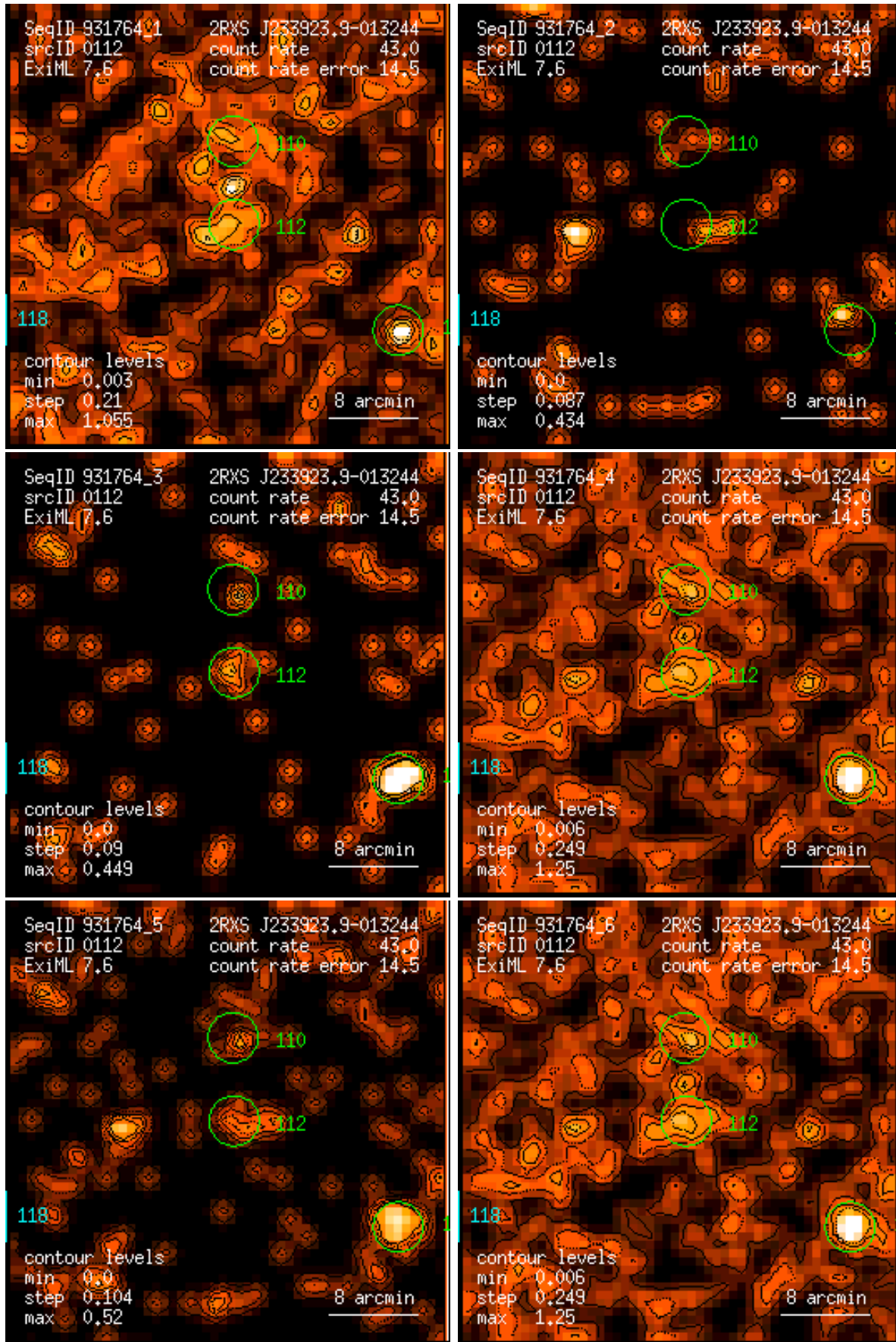
Figure 112: RASS 931764: detection 0112: band rate images, Gaussian filter: (1) PSPC channels 11 – 41, (2) 52 – 90, (3) 91 – 201, (4) 11 – 235, (5) 52 – 201, (6) 11 – 201. Broad band rates in counts/ks. Band rate contour levels in counts/ks/arcmin 2 .
