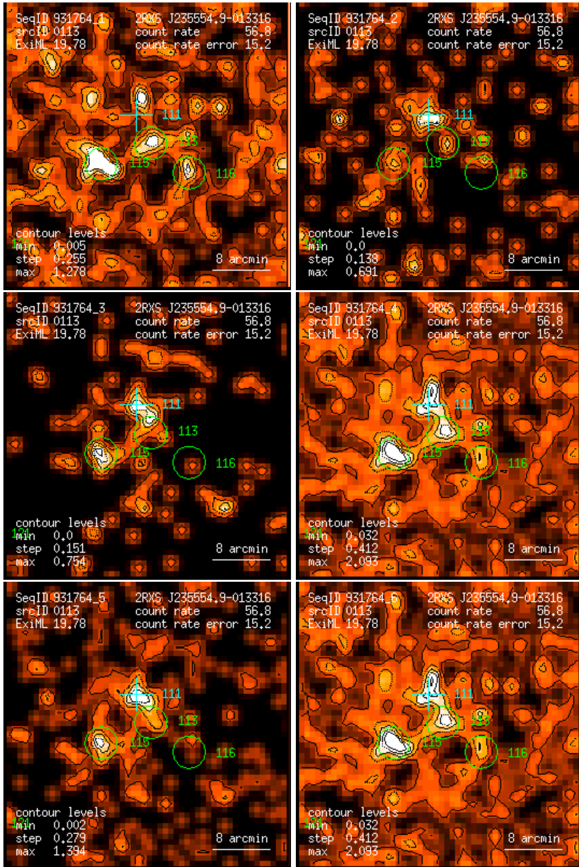
Figure 113: RASS 931764: detection 0113: band rate images, Gaussian filter: (1) PSPC channels 11 – 41, (2) 52 – 90, (3) 91 – 201, (4) 11 – 235, (5) 52 – 201, (6) 11 – 201. Broad band rates in counts/ks. Band rate contour levels in counts/ks/arcmin 2 .
