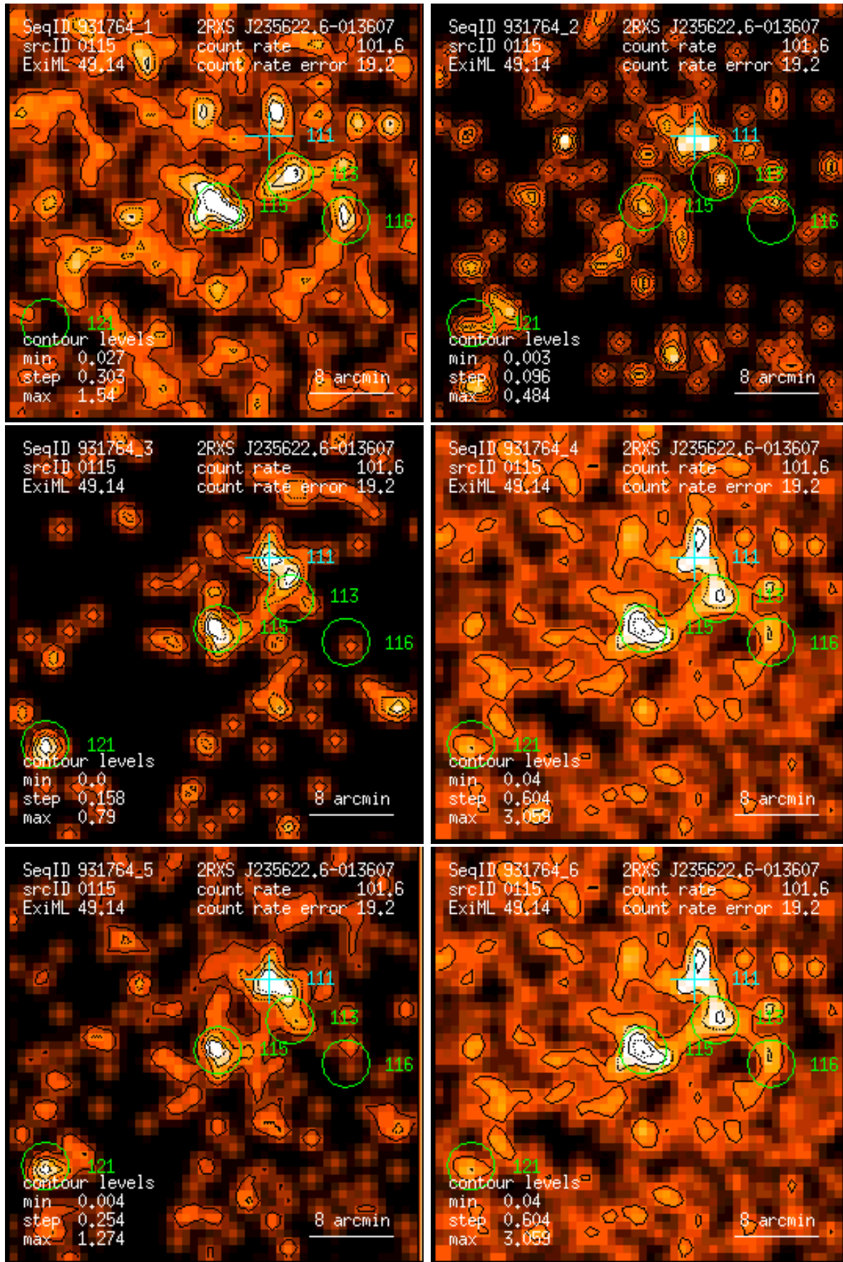
Figure 115: RASS 931764: detection 0115: band rate images, Gaussian filter: (1) PSPC channels 11 – 41, (2) 52 – 90, (3) 91 – 201, (4) 11 – 235, (5) 52 – 201, (6) 11 – 201. Broad band rates in counts/ks. Band rate contour levels in counts/ks/arcmin 2 .
