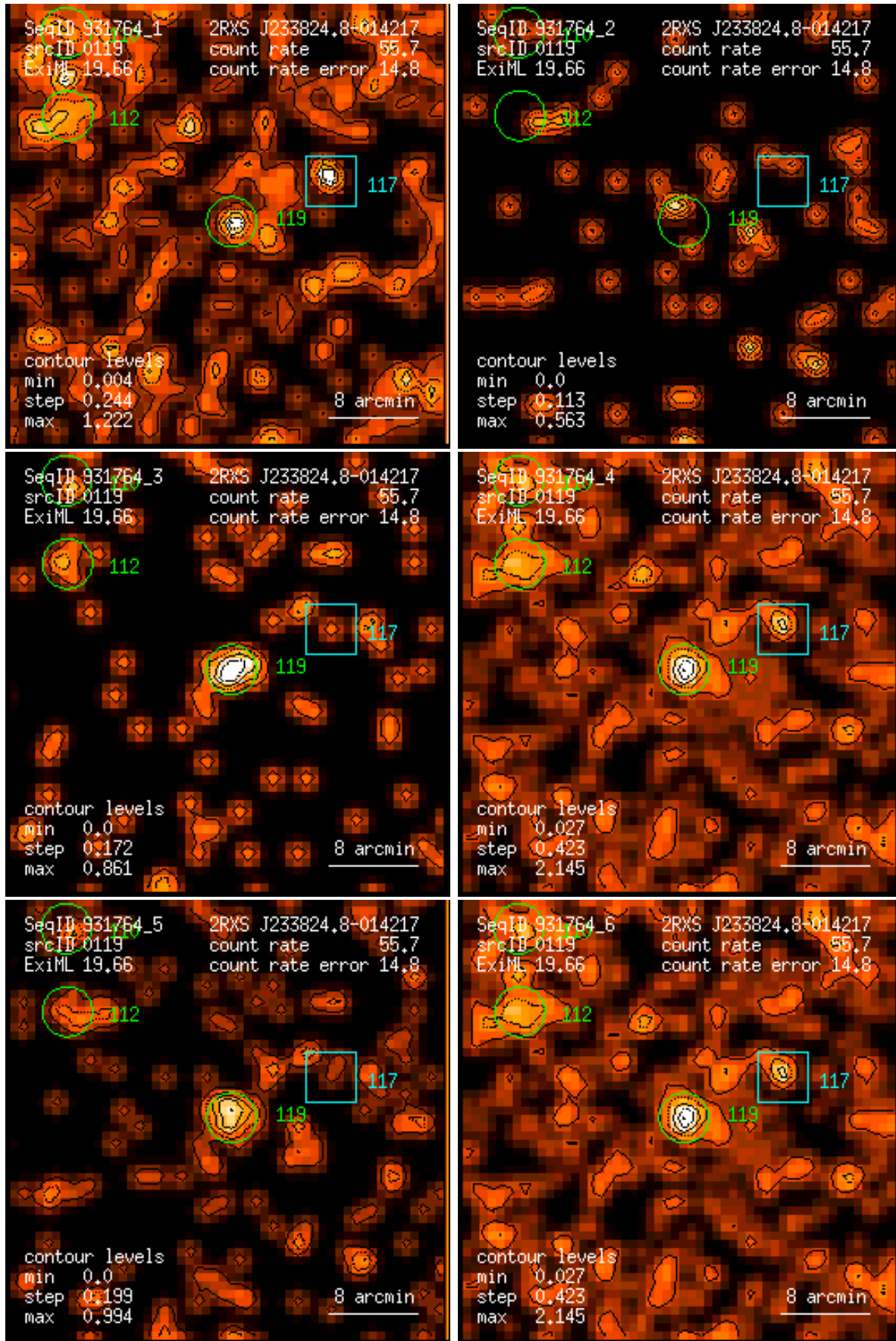
Figure 119: RASS 931764: detection 0119: band rate images, Gaussian filter: (1) PSPC channels 11 – 41, (2) 52 – 90, (3) 91 – 201, (4) 11 – 235, (5) 52 – 201, (6) 11 – 201. Broad band rates in counts/ks. Band rate contour levels in counts/ks/arcmin 2 .
