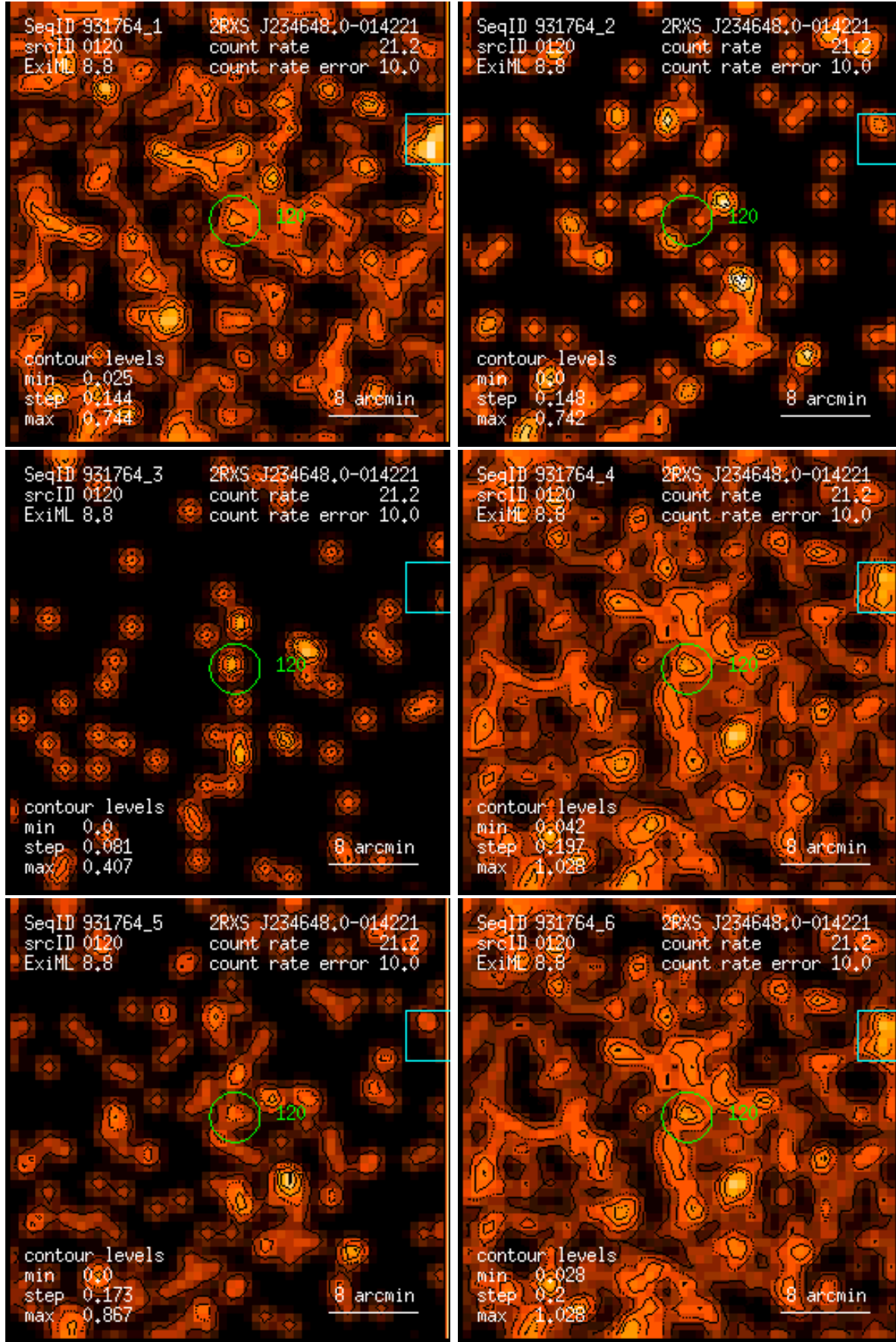
Figure 120: RASS 931764: detection 0120: band rate images, Gaussian filter: (1) PSPC channels 11 – 41, (2) 52 – 90, (3) 91 – 201, (4) 11 – 235, (5) 52 – 201, (6) 11 – 201. Broad band rates in counts/ks. Band rate contour levels in counts/ks/arcmin 2 .
