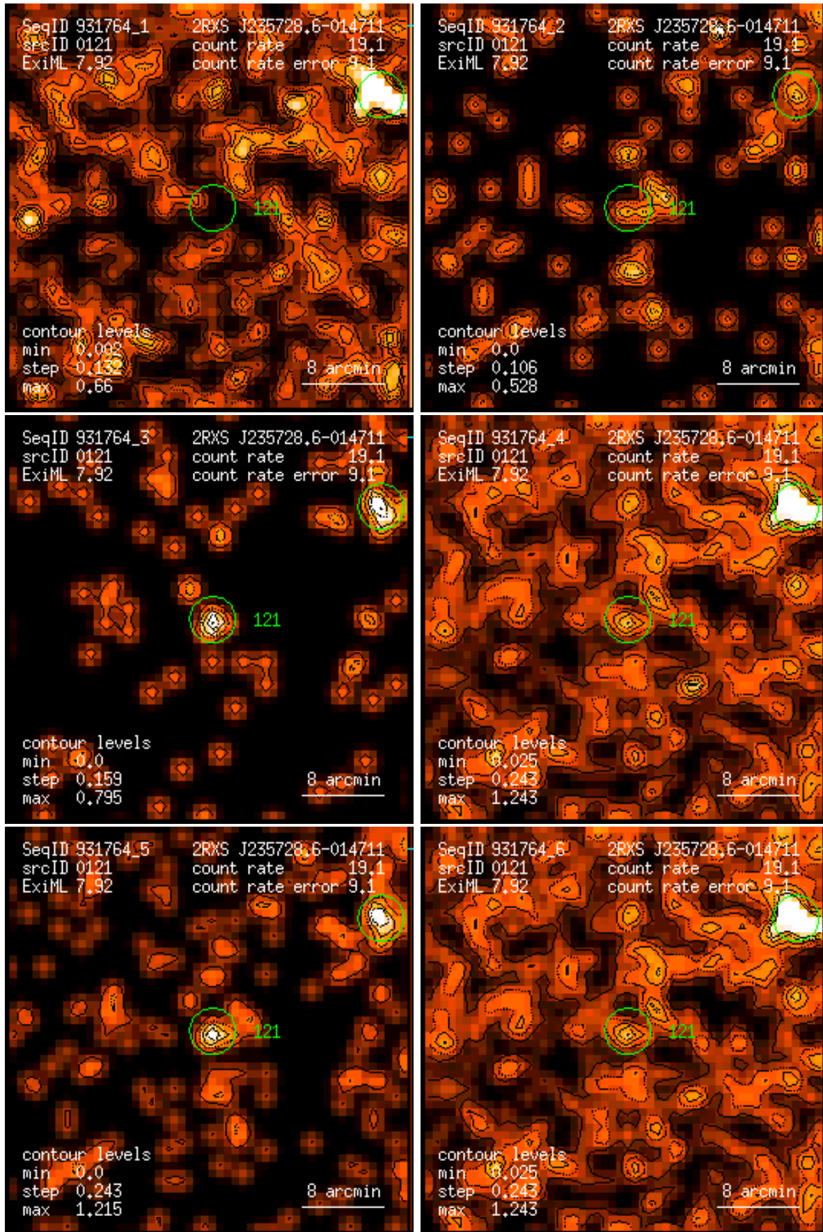
Figure 121: RASS 931764: detection 0121: band rate images, Gaussian filter: (1) PSPC channels 11 – 41, (2) 52 – 90, (3) 91 – 201, (4) 11 – 235, (5) 52 – 201, (6) 11 – 201. Broad band rates in counts/ks. Band rate contour levels in counts/ks/arcmin 2 .
