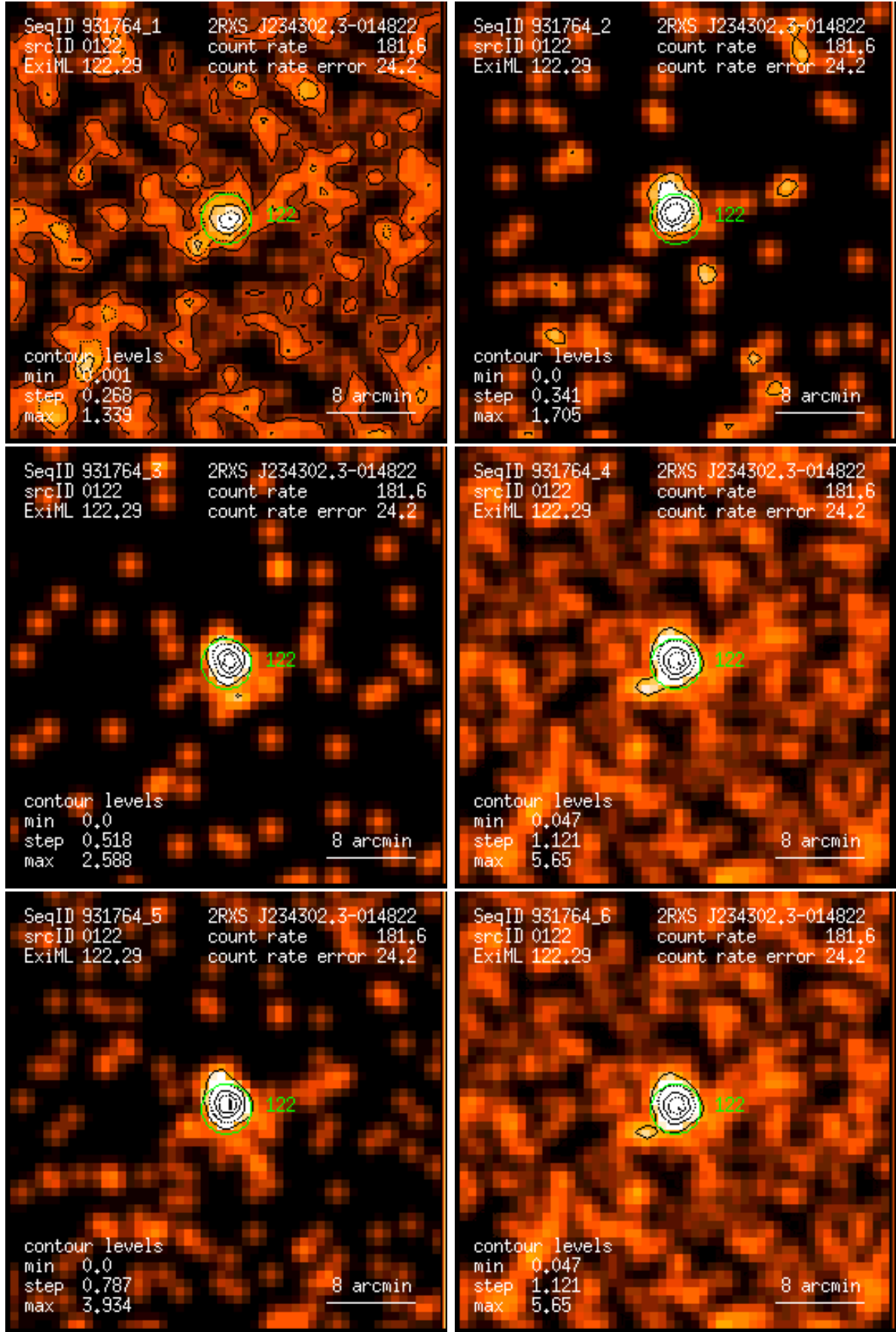
Figure 122: RASS 931764: detection 0122: band rate images, Gaussian filter: (1) PSPC channels 11 – 41, (2) 52 – 90, (3) 91 – 201, (4) 11 – 235, (5) 52 – 201, (6) 11 – 201. Broad band rates in counts/ks. Band rate contour levels in counts/ks/arcmin 2 .
