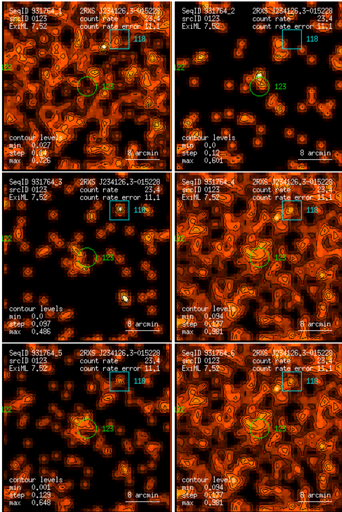
Figure 123: RASS 931764: detection 0123: band rate images, Gaussian filter: (1) PSPC channels 11 – 41, (2) 52 – 90, (3) 91 – 201, (4) 11 – 235, (5) 52 – 201, (6) 11 – 201. Broad band rates in counts/ks. Band rate contour levels in counts/ks/arcmin 2 .
