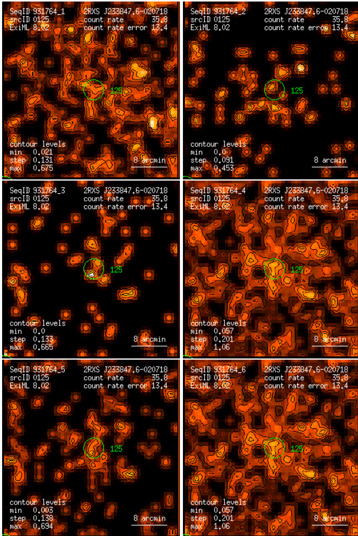
Figure 125: RASS 931764: detection 0125: band rate images, Gaussian filter: (1) PSPC channels 11 – 41, (2) 52 – 90, (3) 91 – 201, (4) 11 – 235, (5) 52 – 201, (6) 11 – 201. Broad band rates in counts/ks. Band rate contour levels in counts/ks/arcmin 2 .
