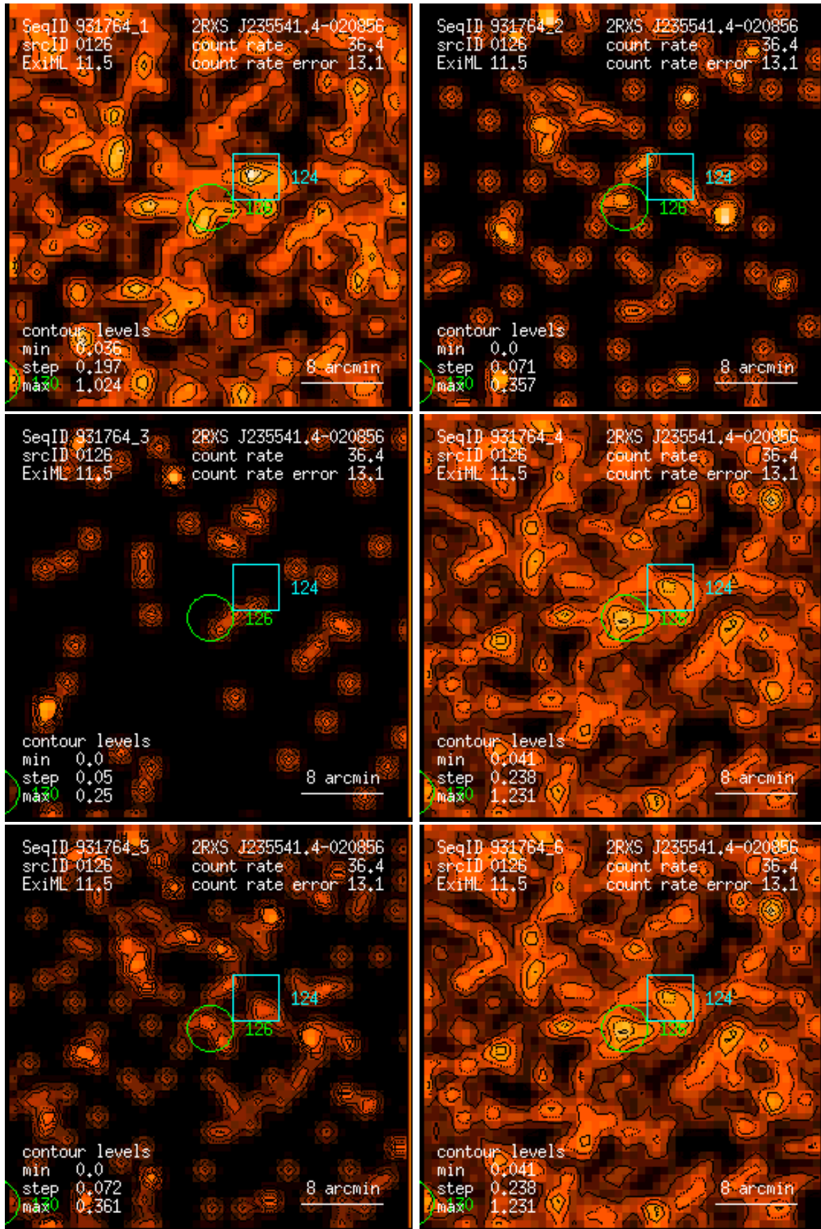
Figure 126: RASS 931764: detection 0126: band rate images, Gaussian filter: (1) PSPC channels 11 – 41, (2) 52 – 90, (3) 91 – 201, (4) 11 – 235, (5) 52 – 201, (6) 11 – 201. Broad band rates in counts/ks. Band rate contour levels in counts/ks/arcmin 2 .
