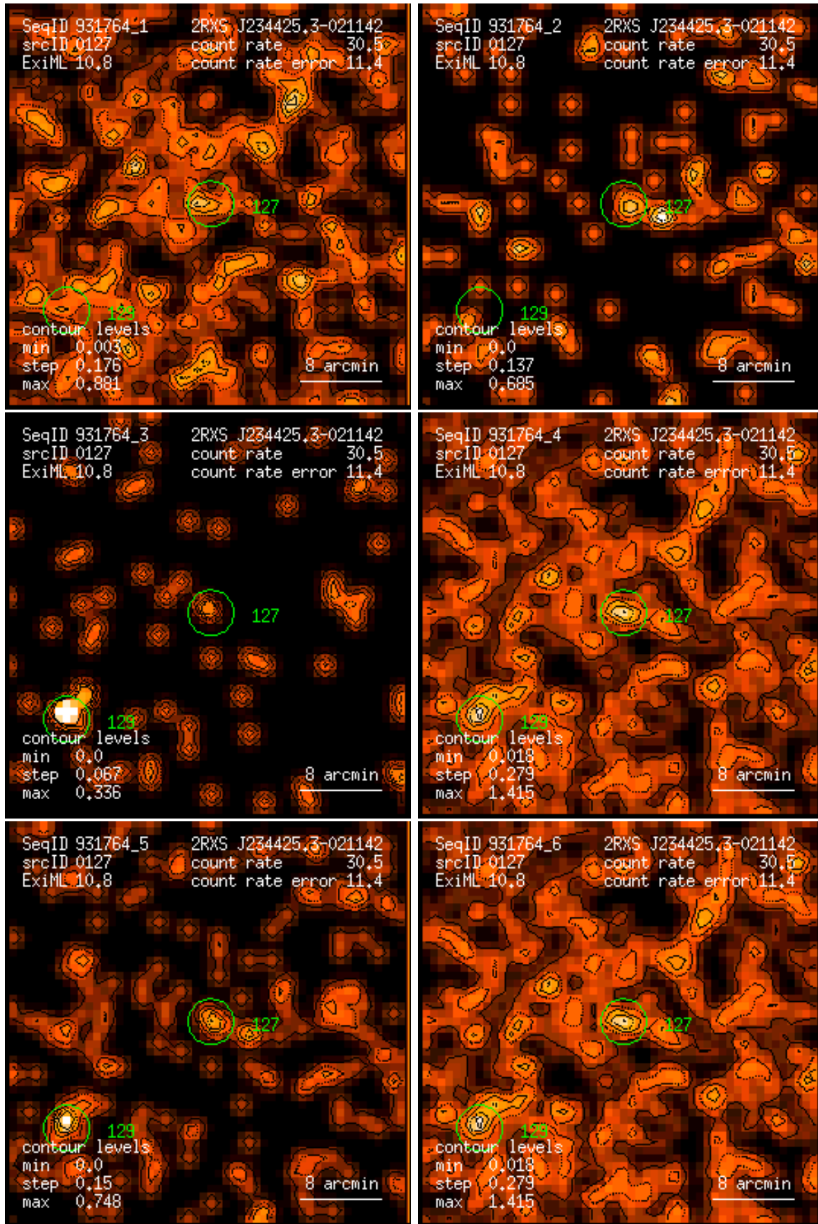
Figure 127: RASS 931764: detection 0127: band rate images, Gaussian filter: (1) PSPC channels 11 – 41, (2) 52 – 90, (3) 91 – 201, (4) 11 – 235, (5) 52 – 201, (6) 11 – 201. Broad band rates in counts/ks. Band rate contour levels in counts/ks/arcmin 2 .
