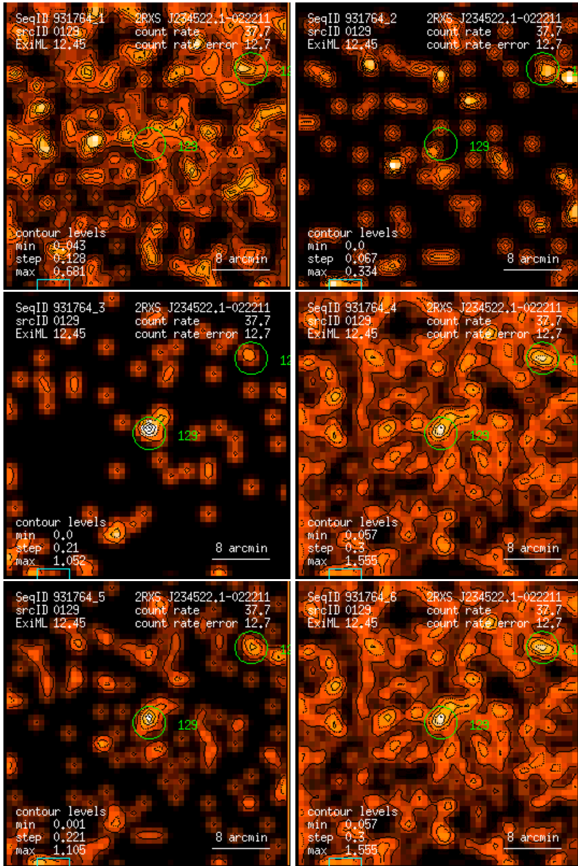
Figure 129: RASS 931764: detection 0129: band rate images, Gaussian filter: (1) PSPC channels 11 – 41, (2) 52 – 90, (3) 91 – 201, (4) 11 – 235, (5) 52 – 201, (6) 11 – 201. Broad band rates in counts/ks. Band rate contour levels in counts/ks/arcmin 2 .
